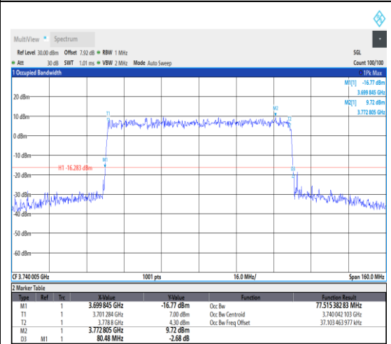
1-N77-3700-3980--30-80-L-9-CP-256QAM-Outer_Full-217@0-Ant1-77.515-80.480-≤80-PASS
