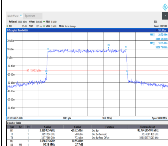
1-N77-3700-3980--30-90-H-5-DFT-256QAM-
