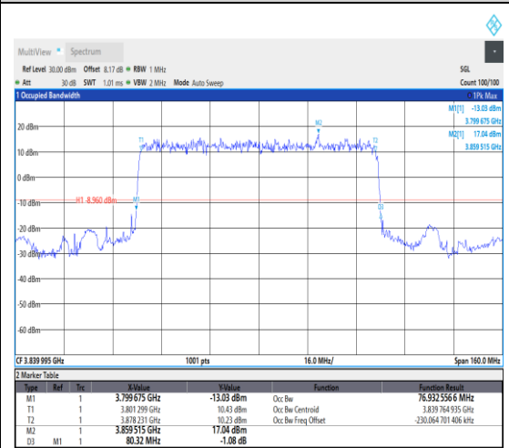
1-N77-3700-3980--30-80-M-2-DFT-PI2BPSK-Outer_Full-217@0-Ant1-77.515-80.480-≤80-PASS
