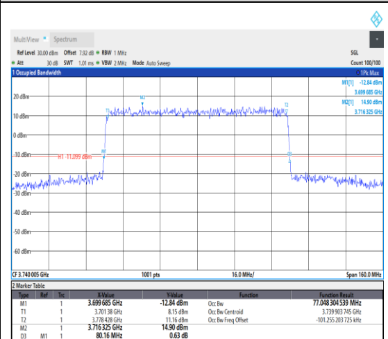
1-N77-3700-3980--30-80-L-1-DFT-QPSK-Out
