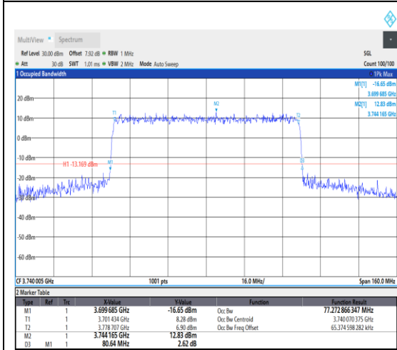
1-N77-3700-3980--30-80-L-8-CP-64QAM-Outer_Full-217@0-Ant1-77.273-80.640-≤80-PASS
