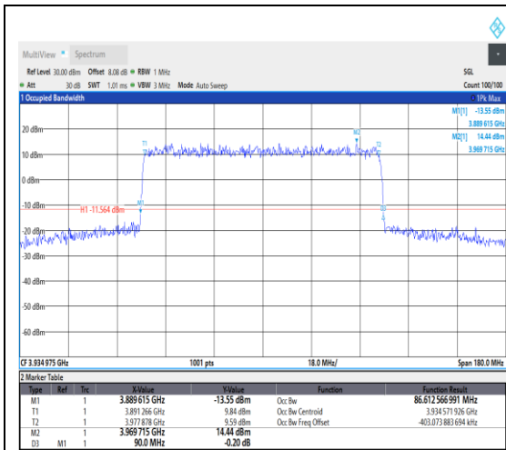
1-N77-3700-3980--30-90-H-1-DFT-QPSK-Outer_Full-243@0-Ant1-86.613-90.000-≤90-PA SS
