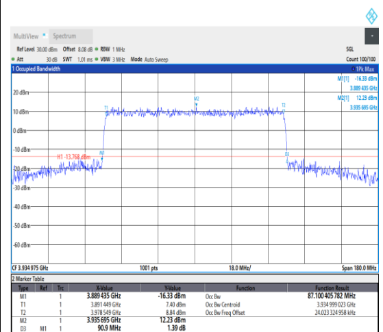
1-N77-3700-3980--30-90-H-6-CP-QPSK-Out
