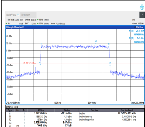
1-N77-3700-3980--30-100-H-9-CP-256QAM-
