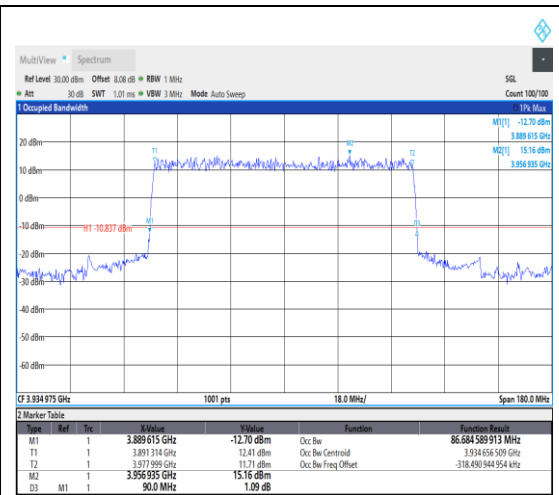
1-N77-3700-3980--30-90-H-2-DFT-PI2BPSK-Outer_Full-243@0-Ant1-86.685-90.000-≤90-PASS
