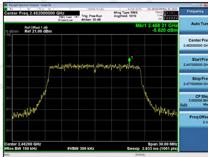
11G-Ant1-2462-0~Reference-PASS
