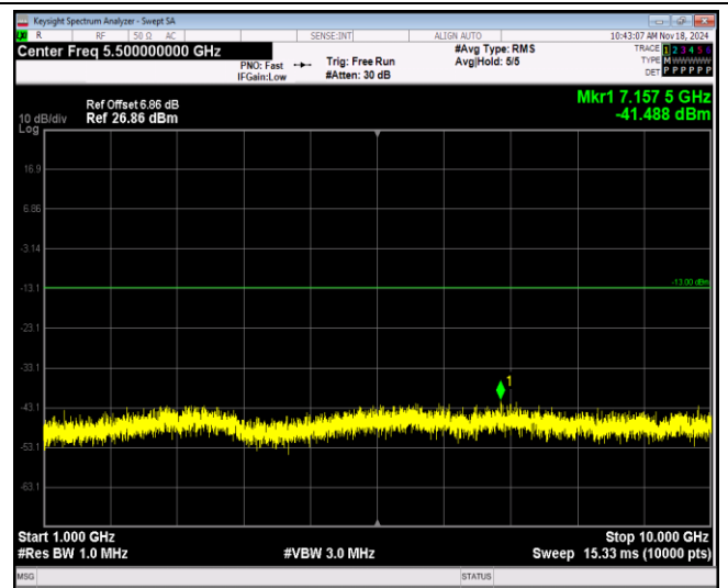
Band26-10MHz-64QAM-26740-1RB#0-Range2:1000~10000MHz
