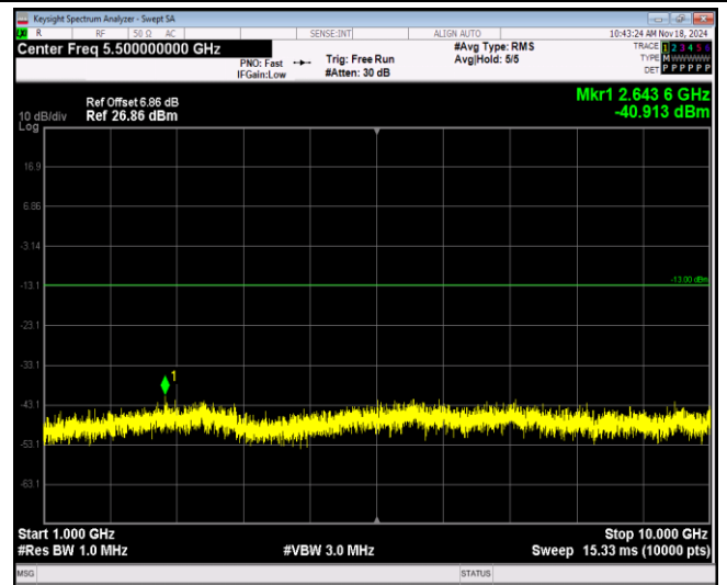
Band26-15MHz-QPSK-26865-1RB#0-Range2:1000~10000MHz
