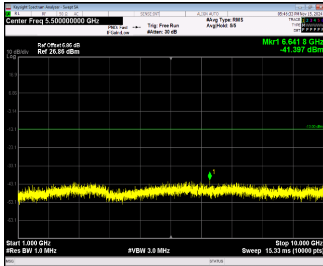
Band17-5MHz-64QAM-23755-1RB#0-Range2:1000~10000MHz
