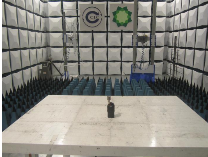
Radiated Emission:
