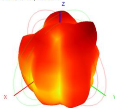
2400.0MHz H+V, Eff: 51.0%
