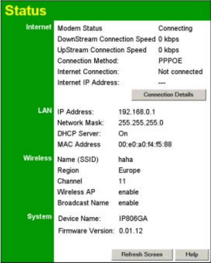
Figure 23: Status Screen
