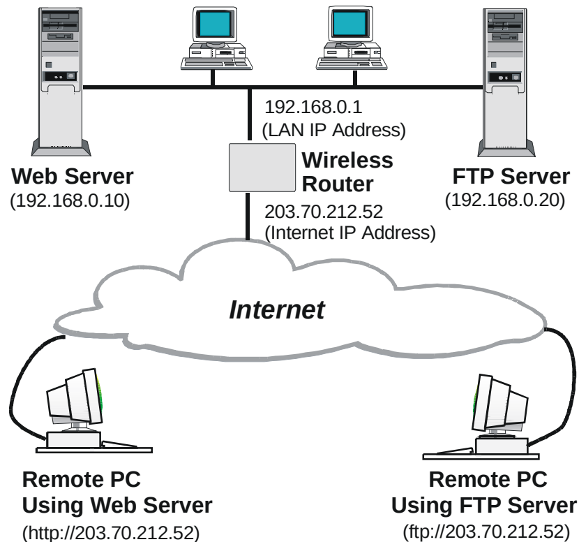
Figure 35: Virtual Servers
