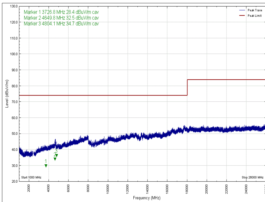
Figure 18 - 2402 MHz - 1 GHz to 26 GHz, Polarity: Horizontal, EUT Orientation: Y, Peak
