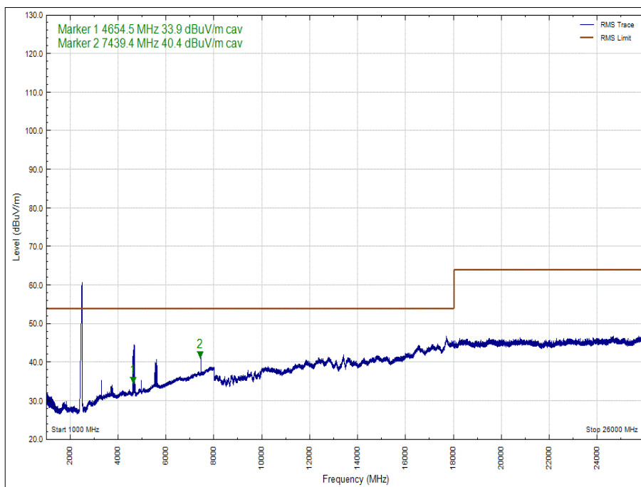
Figure 56 - 2480 MHz - 1 GHz to 26 GHz, Polarity: Horizontal, EUT Orientation: Y, Average
