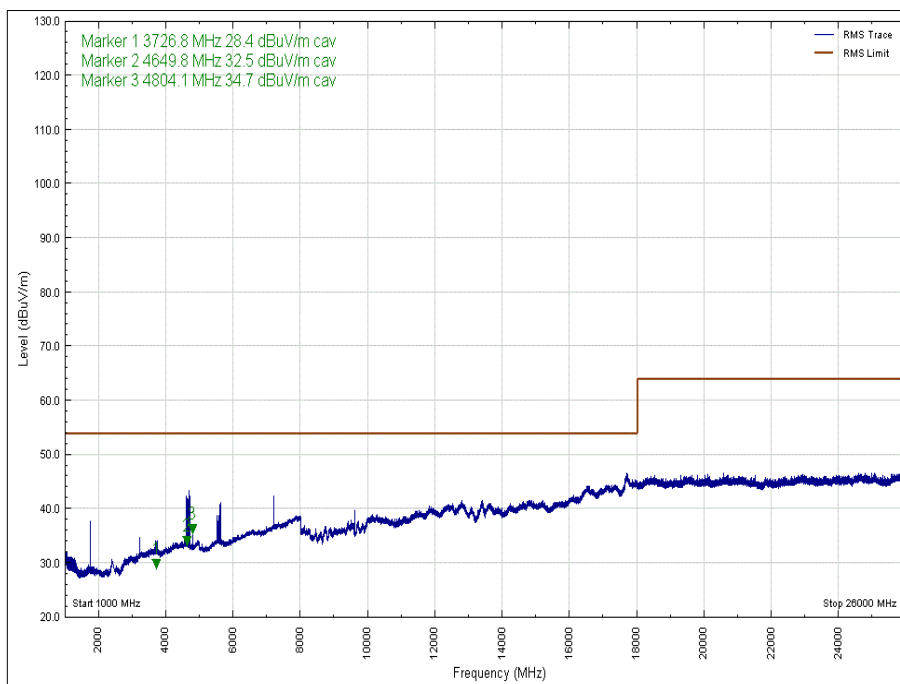
Figure 20 - 2402 MHz - 1 GHz to 26 GHz, Polarity: Horizontal, EUT Orientation: Y, Average
