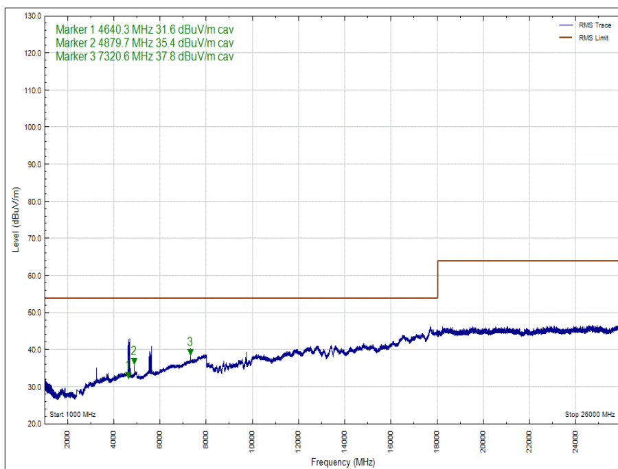
Figure 38 - 2441 MHz - 1 GHz to 26 GHz, Polarity: Horizontal, EUT Orientation: Y, Average
