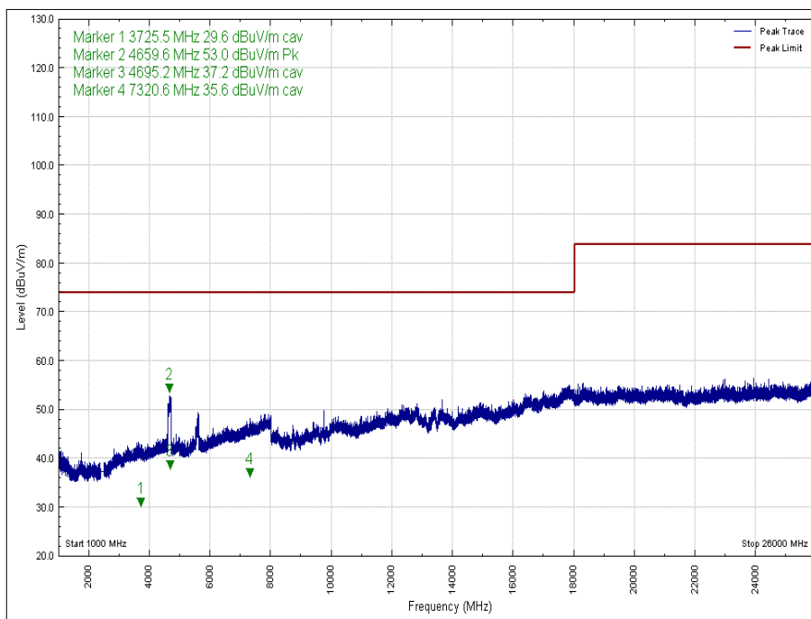
Figure 39 - 2441 MHz - 1 GHz to 26 GHz, Polarity: Vertical, EUT Orientation: Z, Peak
