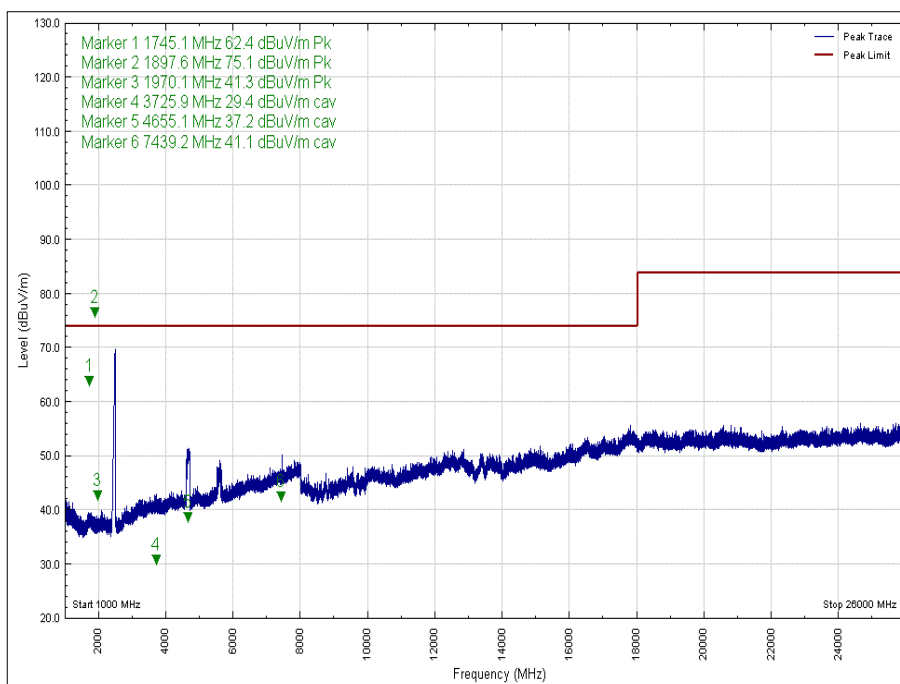
Figure 57 - 2480 MHz - 1 GHz to 26 GHz, Polarity: Vertical, EUT Orientation: Z, Peak
