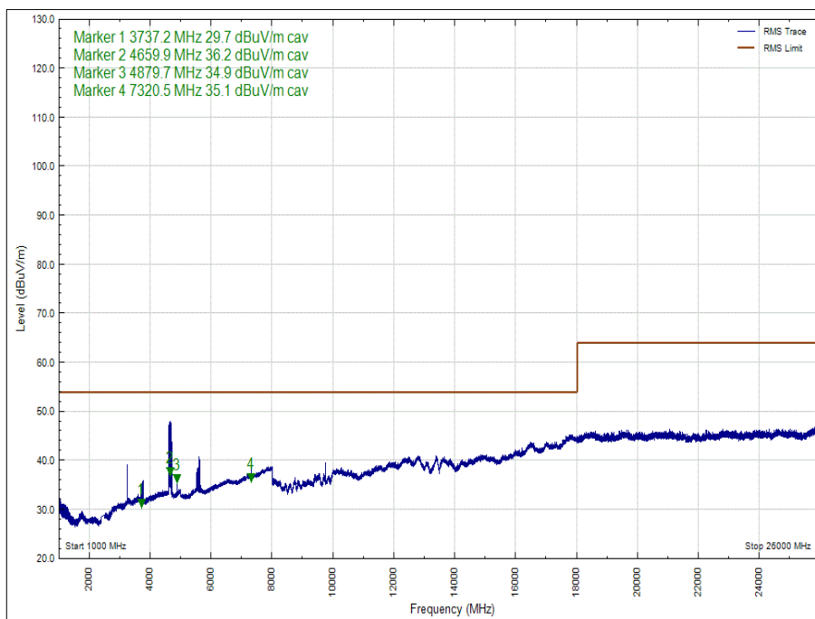
Figure 37 - 2441 MHz - 1 GHz to 26 GHz, Polarity: Vertical, EUT Orientation: Y, Average
