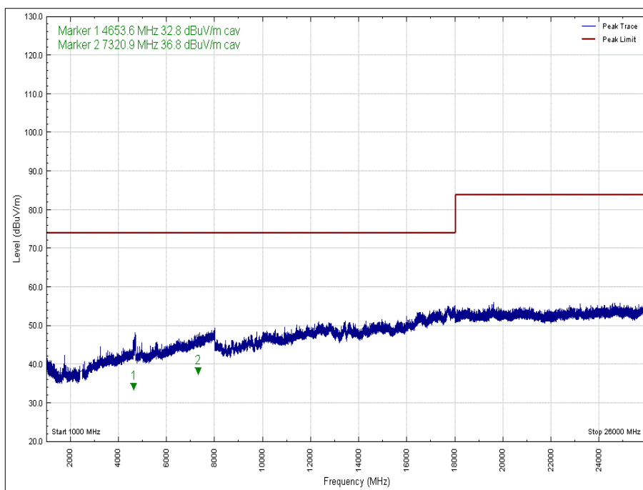
Figure 40 - 2441 MHz - 1 GHz to 26 GHz, Polarity: Horizontal, EUT Orientation: Z, Peak
