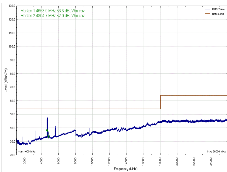
Figure 19 - 2402 MHz - 1 GHz to 26 GHz, Polarity: Vertical, EUT Orientation: Y, Average
