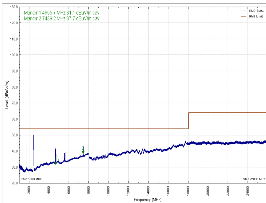
Figure 60 - 2480 MHz - 1 GHz to 26 GHz, Polarity: Horizontal, EUT Orientation: Z, Average
