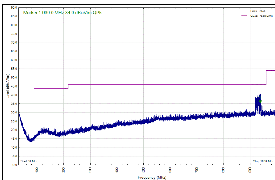
Figure 26 - 30 MHz to 1 GHz, 2441 MHz, Polarity: Horizontal, EUT Orientation X
