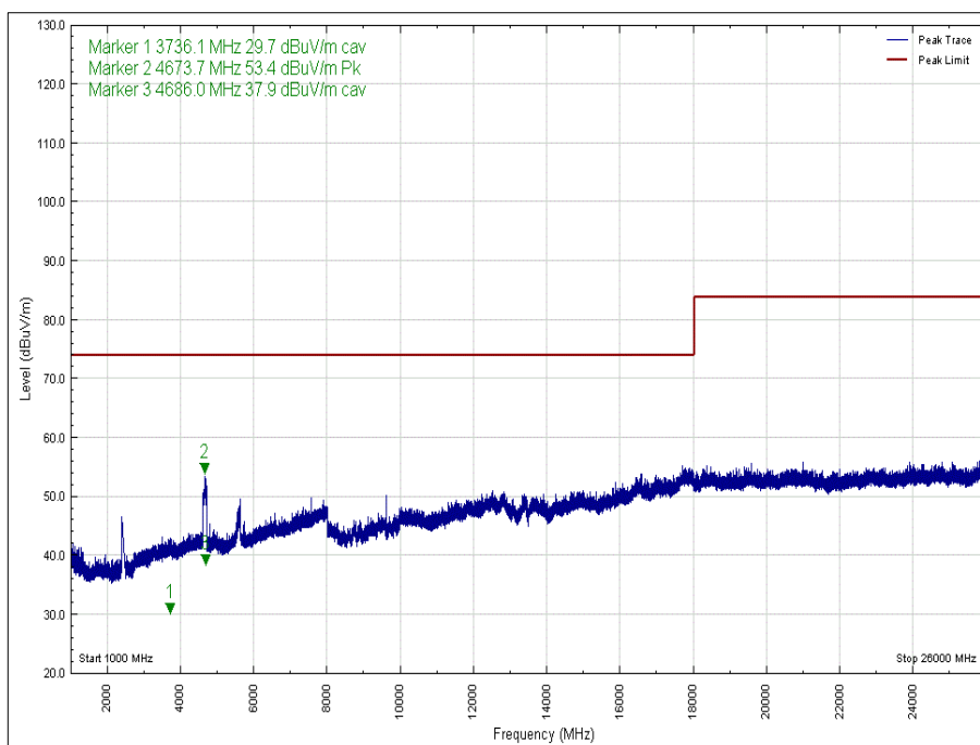
Figure 21 - 2402 MHz - 1 GHz to 26 GHz, Polarity: Vertical, EUT Orientation: Z, Peak
