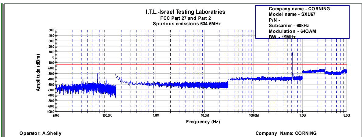
Figure 678: Spurious Emissions at Antenna Terminal 64QAM, 634.5MHz, B.W. 15MHz, Sub Carrier 60kHz
