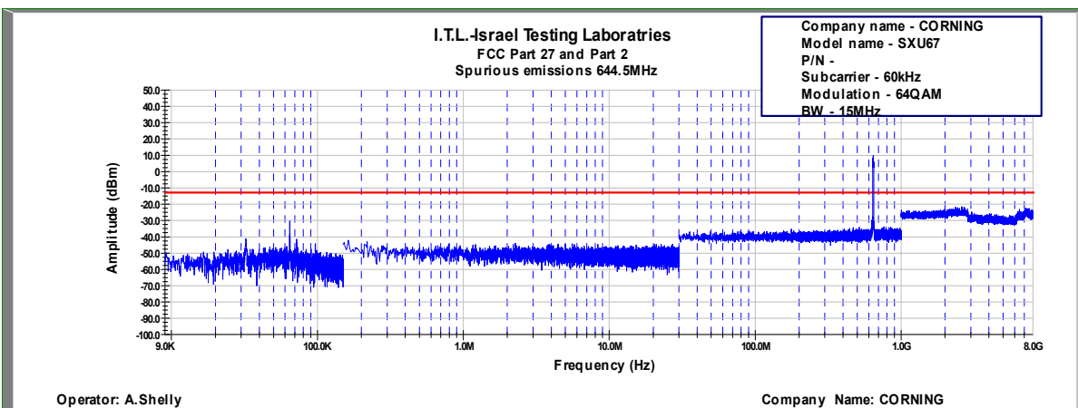
Figure 679: Spurious Emissions at Antenna Terminal 64QAM, 644.5MHz, B.W. 15MHz, Sub Carrier 60kHz
