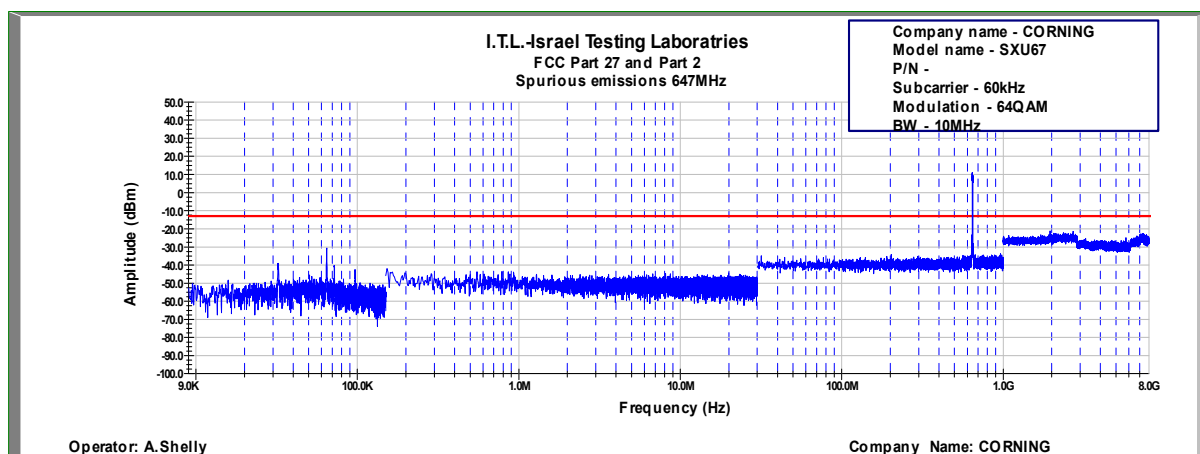
Figure 670: Spurious Emissions at Antenna Terminal 64QAM, 647.0MHz, B.W. 10MHz, Sub Carrier 60kHz
