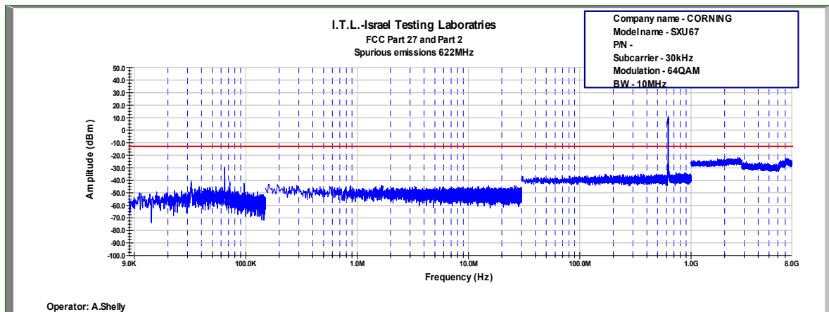
Figure 665: Spurious Emissions at Antenna Terminal 64QAM, 622.0MHz, B.W. 10MHz, Sub Carrier 30kHz
