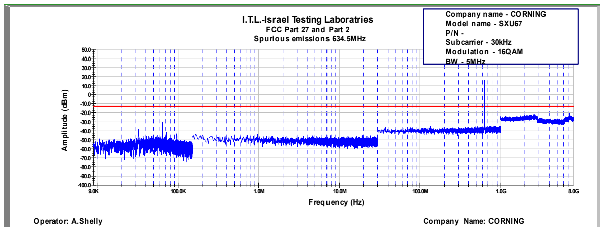
Figure 627: Spurious Emissions at Antenna Terminal 16QAM, 634.5MHz, B.W. 5MHz, Sub Carrier 30kHz
