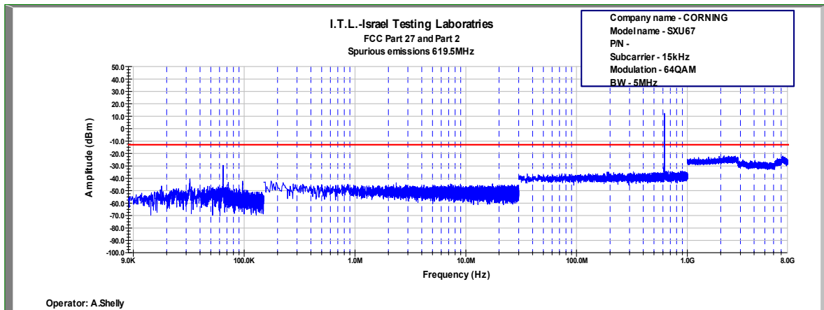
Figure 656: Spurious Emissions at Antenna Terminal 64QAM, 619.5MHz, B.W. 5MHz, Sub Carrier 15kHz
