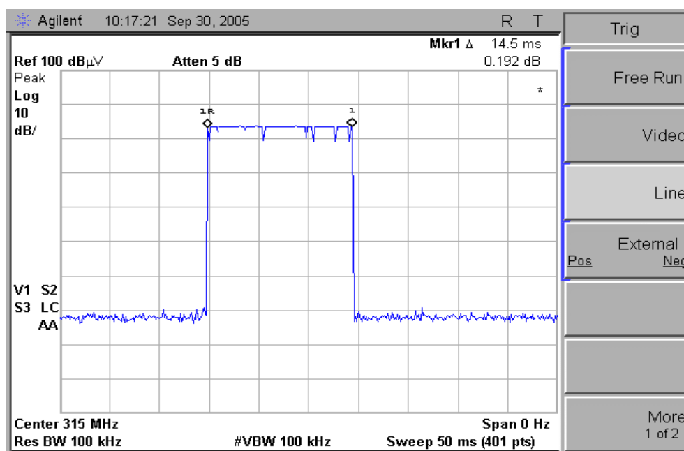
Figure 1. normal transmission
