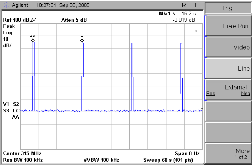
Figure 4. Transmission interval
