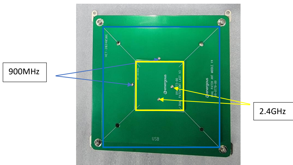
Antenna Top View w/ Frame
