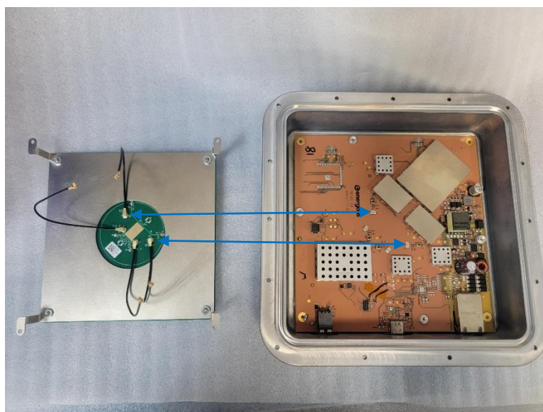
PCB and Antenna U.FL connections Top View 900MHz
