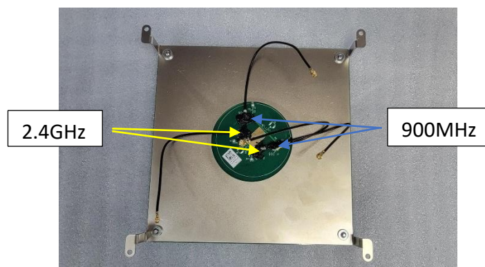
Antenna Bottom View w/ Frame
