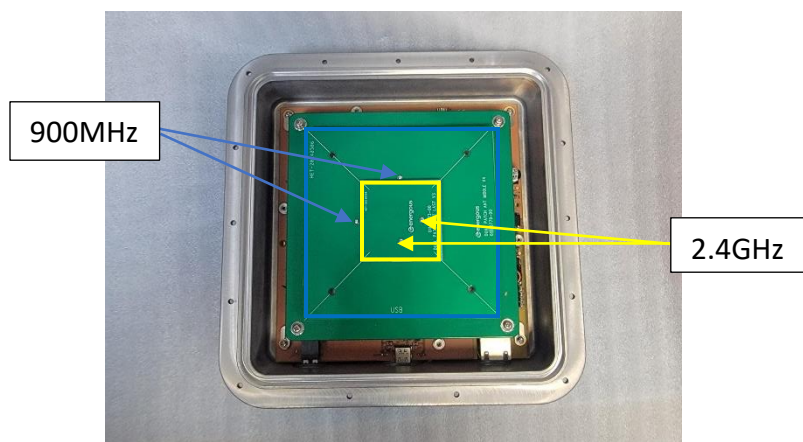
PCB and Antenna U.FL connections Top View 900MHz
