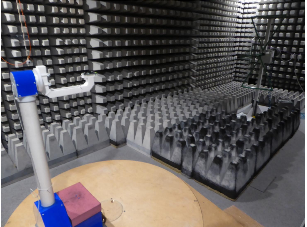
Test setup fully anechoic chamber 30 MHz – 1 GHz
