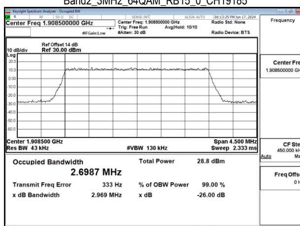
Band2_3MHz_64QAM_RB15_0_CH19185
