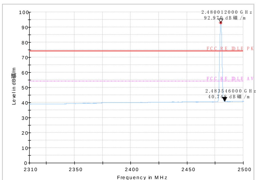
Fig.29 Bandedge:CH39
