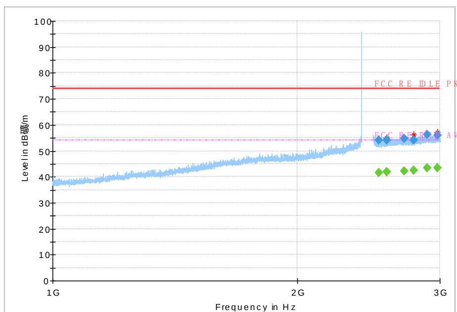
Fig.19 Radiated emission: CH0, 1GHz~3GHz
