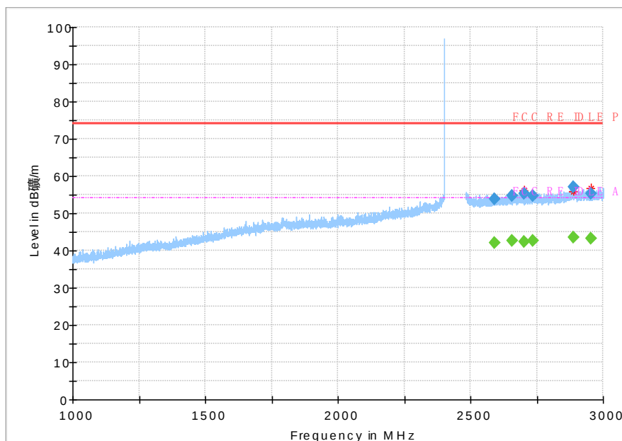
Fig.27 Radiated emission: CH39, 1GHz~3GHz
