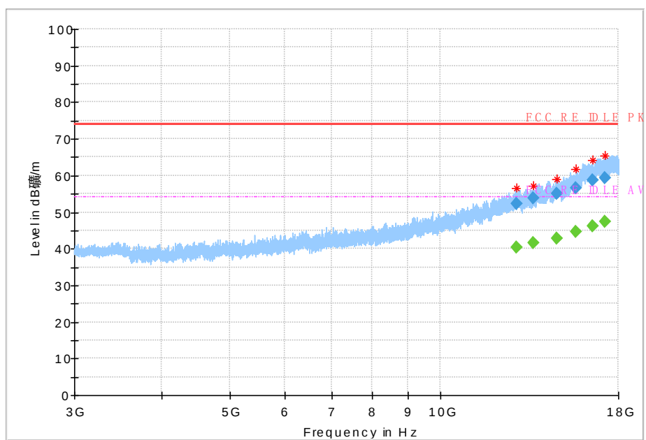
Fig.20 Radiated emission: CH0, 3GHz~18GHz
