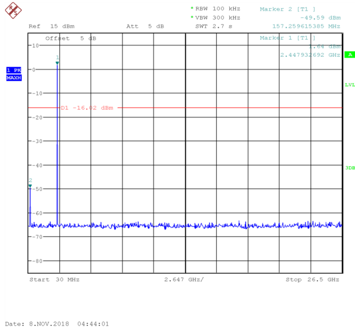
Fig.17 Conducted spurious emission: Ch39, 30MHz~26GHz
