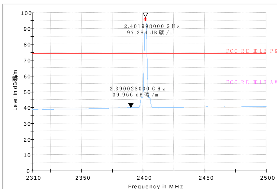
Fig.21 Bandedge: CH0
