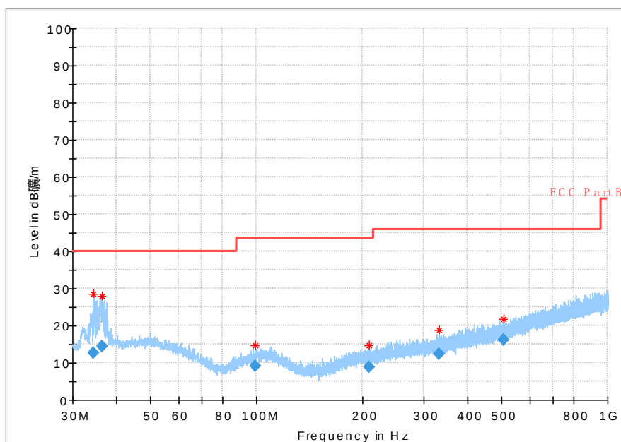
Fig.26 Radiated emission: CH39, 30MHz~1GHz
