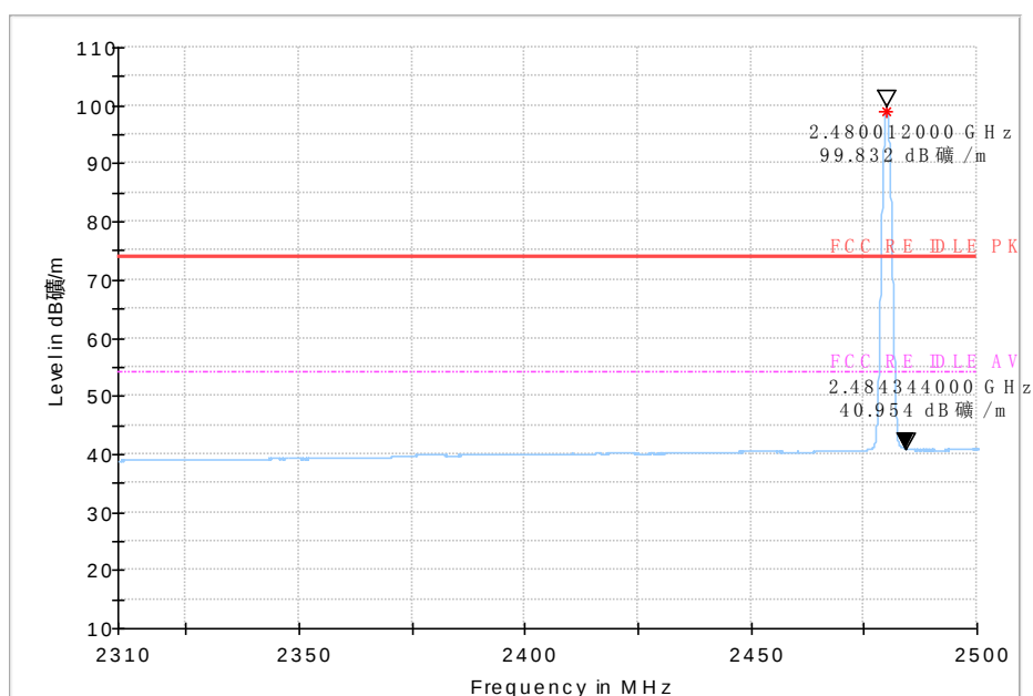
Fig.25 Bandedge:CH39
