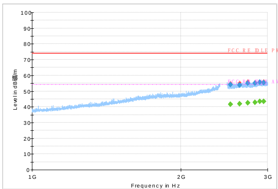
Fig.23 Radiated emission: CH39, 1GHz~3GHz
