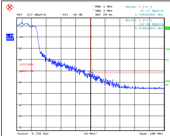
Band Edge 5725 MHz, ch136, 802.11n HT20 MIMO, Radiated, Max, Pk PL12
