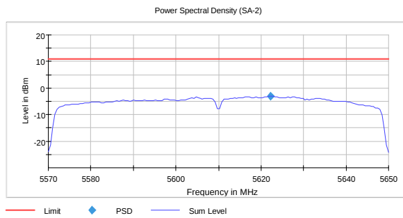
PSD, 5610 MHz, 802.11ac, HT80, Ant1, -3.1
