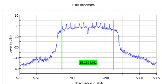
DTS BW, 5785 MHz, 802.11n, HT20
