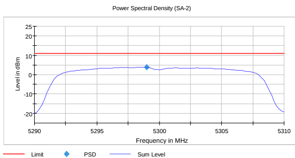
PSD, 5300 MHz, 802.11a, 6Mb 3.8
