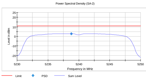
PSD, 5240 MHz, 802.11a, 6Mb 2.9
