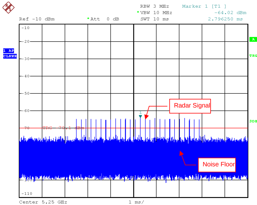
Radar Signal 2
