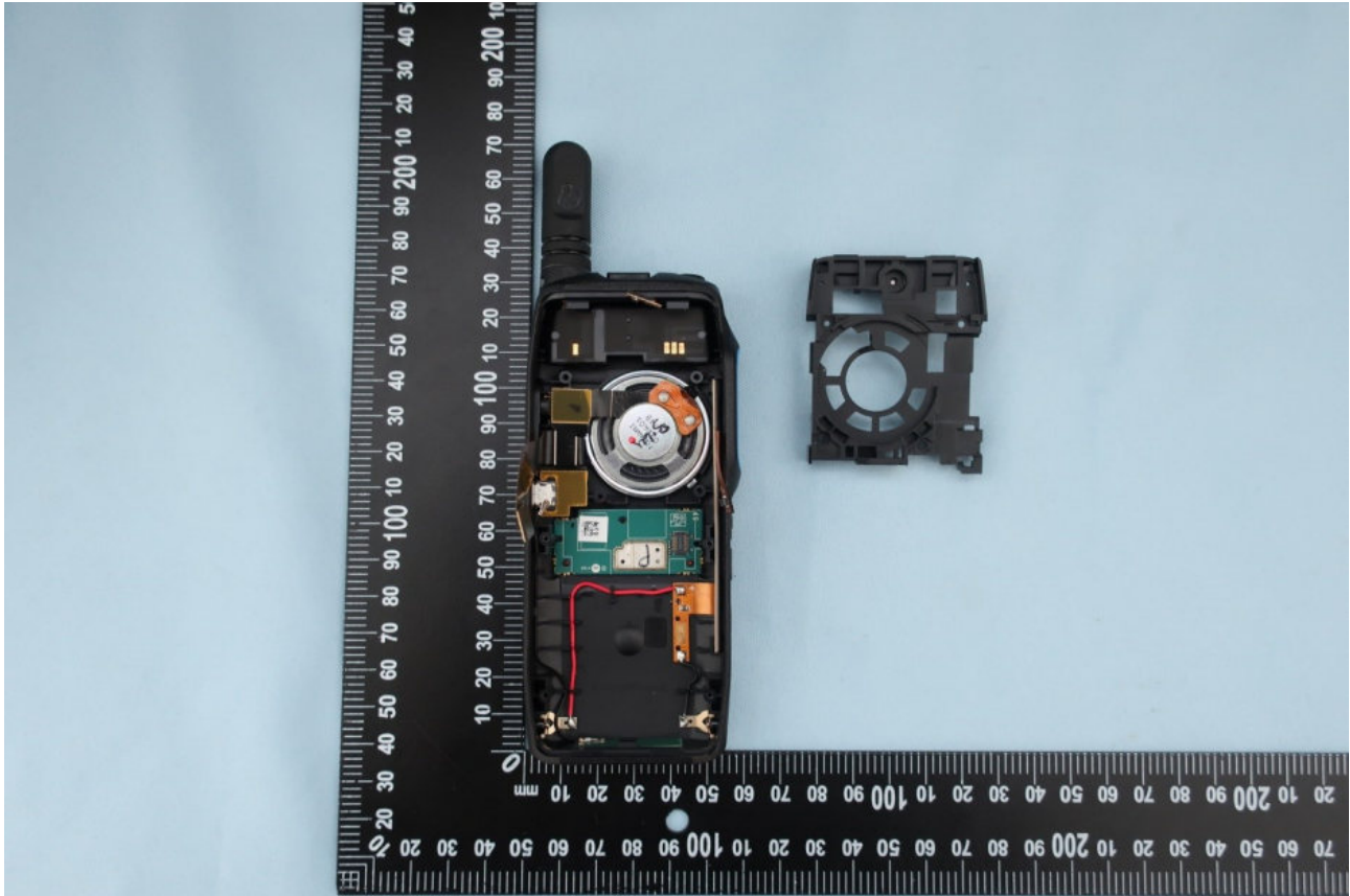
<Device disassembled speaker frame>
