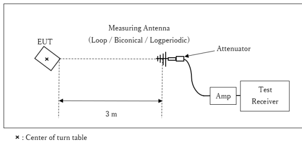
Figure 2: Test Setup
