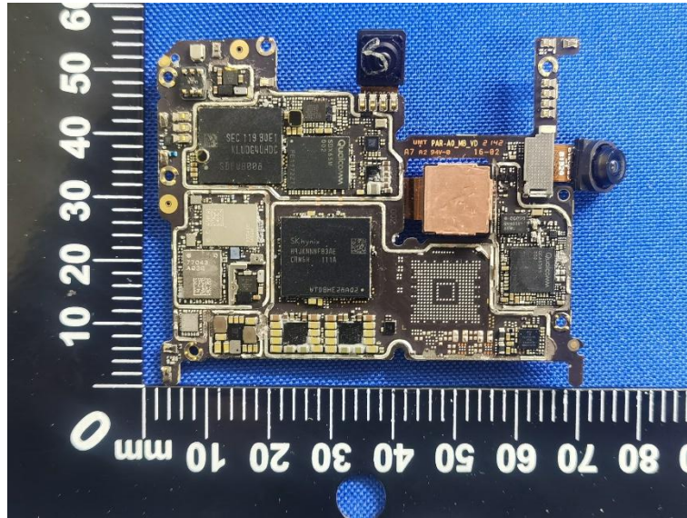
MAIN BOARD REAR VIEW
