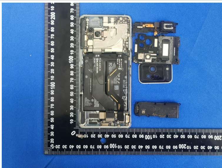
EUT UNCOVER VIEW 2
