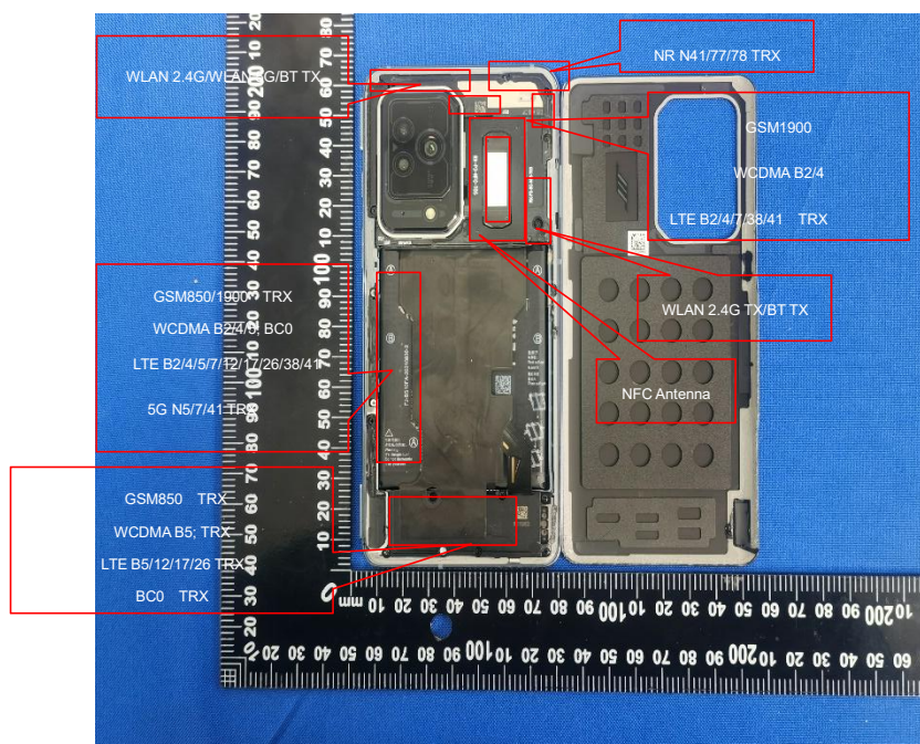
EUT UNCOVER VIEW 1
