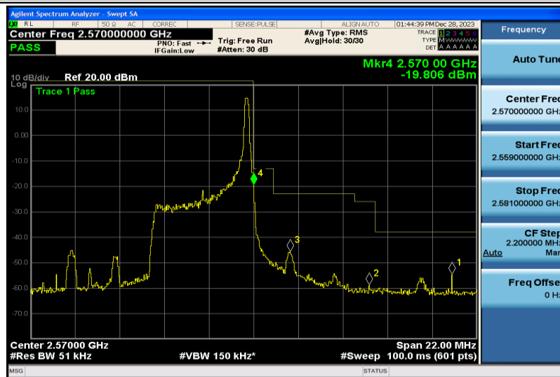
Band7-5MHz-16QAM-21425-1RB#24
