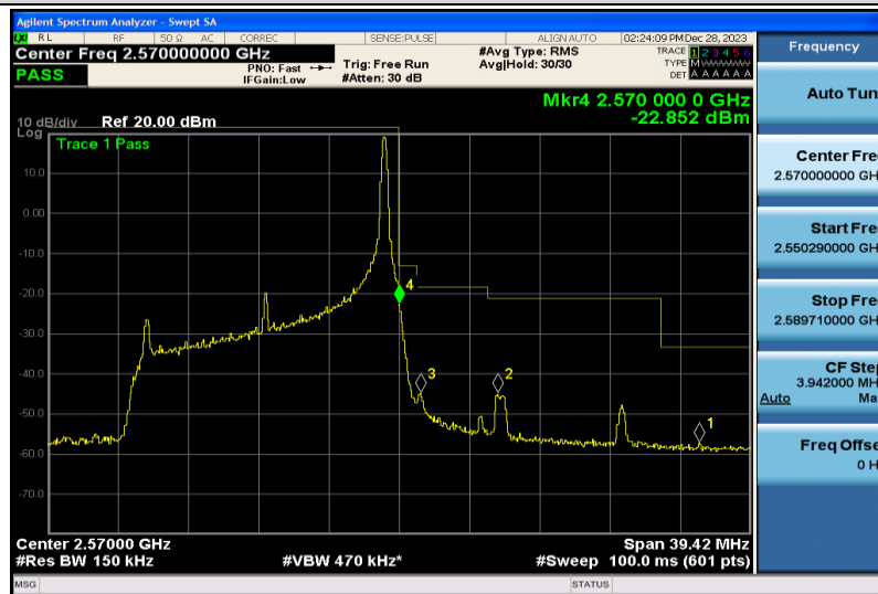
Band7-15MHz-QPSK-21375-1RB#74
