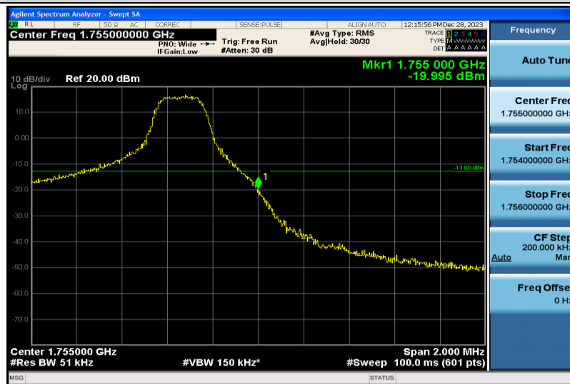
Band4-5MHz-QPSK-20375-1RB#24
