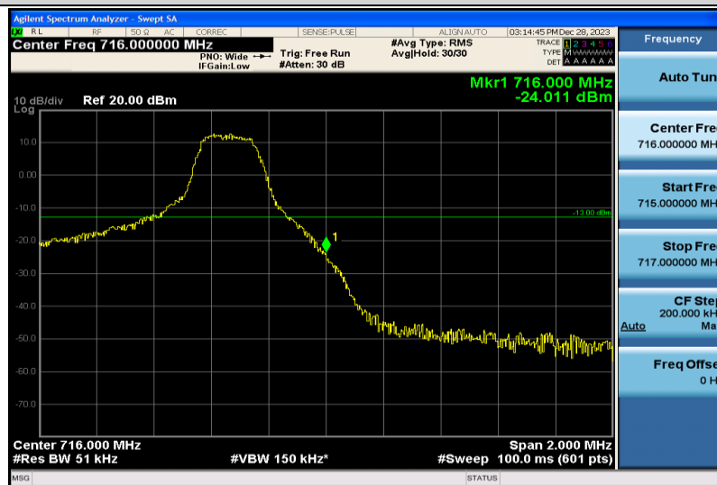
Band17-5MHz-QPSK-23825-1RB#24
