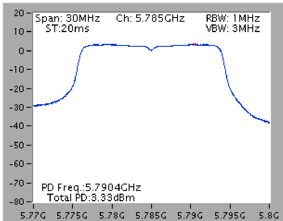
Power Density Plot on Configuration IEEE 802.11ac MCS0/Nss1 VHT20 / Chain 2 / 5785 MHz
