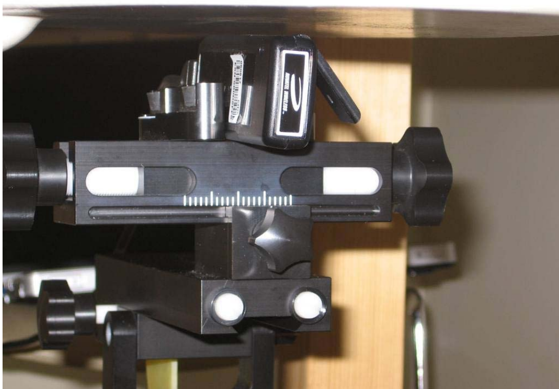
Figure 13: Right Edge - Antenna at 45 Degrees
