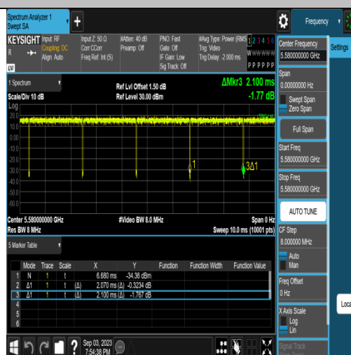
NTNV-11A-Ant1-5580
