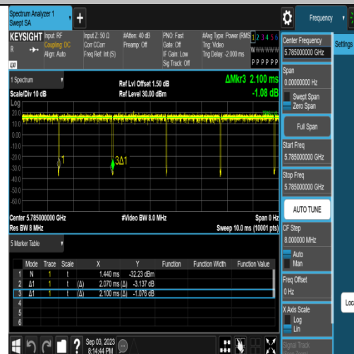
NTNV-11A-Ant1-5785
