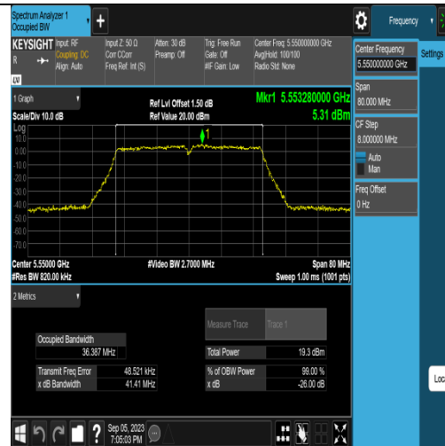
11AC40SISO-Ant1-5550
