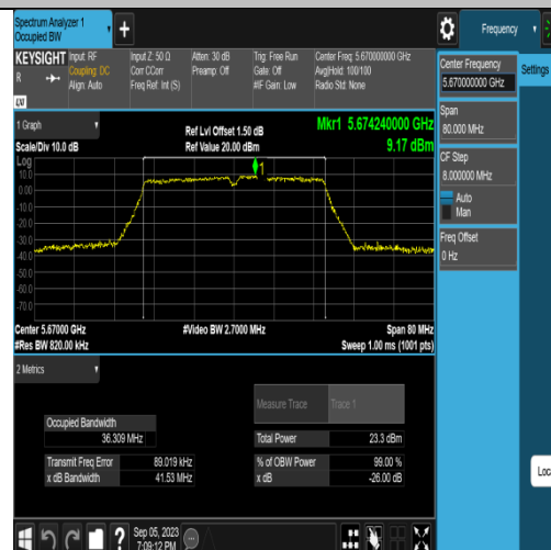
11AC40SISO-Ant1-5670
