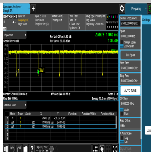
NTNV-11N20SISO-Ant1-5500
