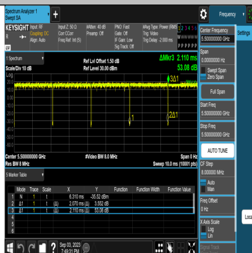
NTNV-11A-Ant1-5500
