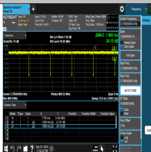
NTNV-11N20SISO-Ant1-5785
