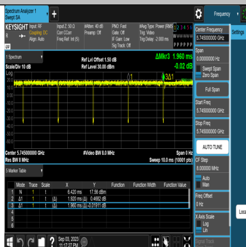
NTNV-11N20SISO-Ant1-5745
