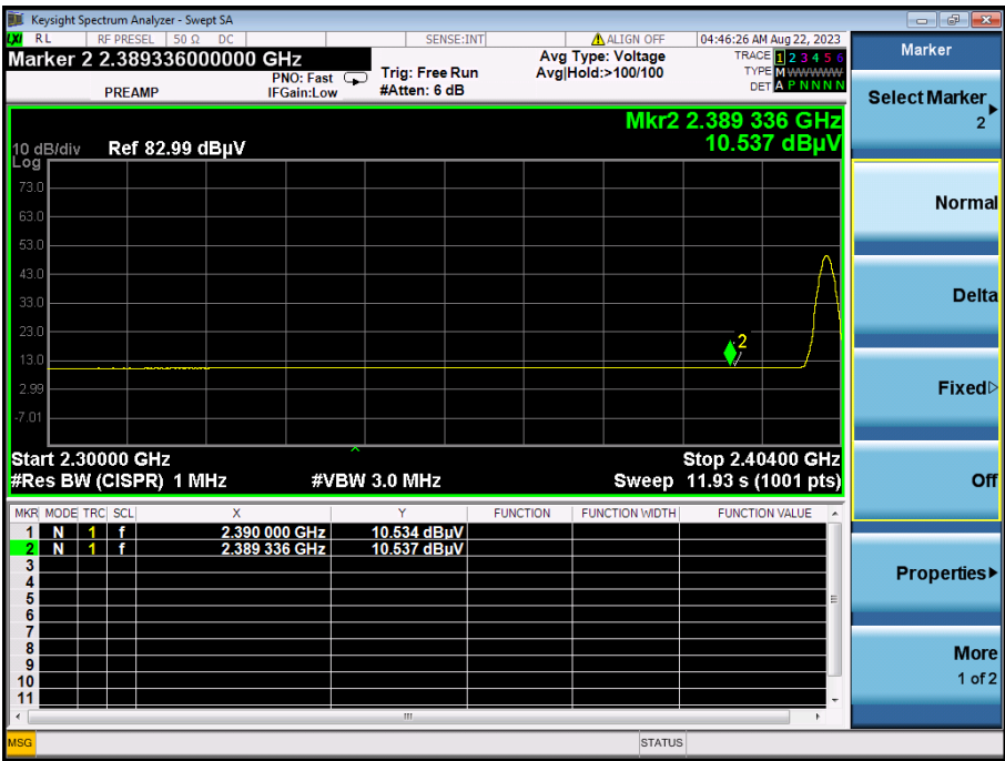
(AVERAGE, Channel 0)
