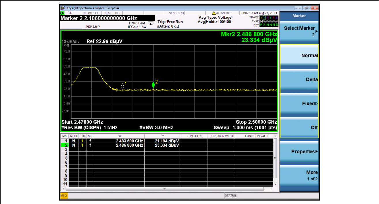
(PEAK, Channel 39)
