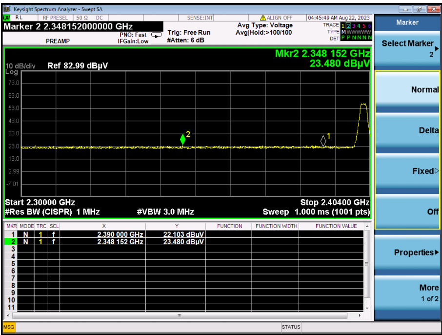
(PEAK, Channel 0)
