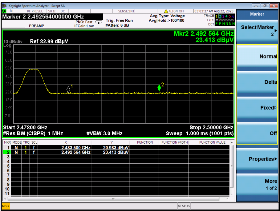
(PEAK, Channel 39)
