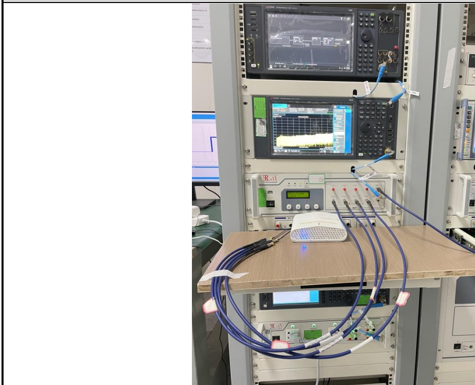
DFS Test Setup
