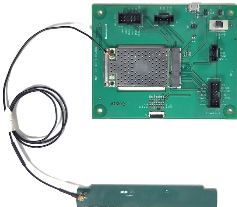
RFID Coupler, RFID module and Test Board
