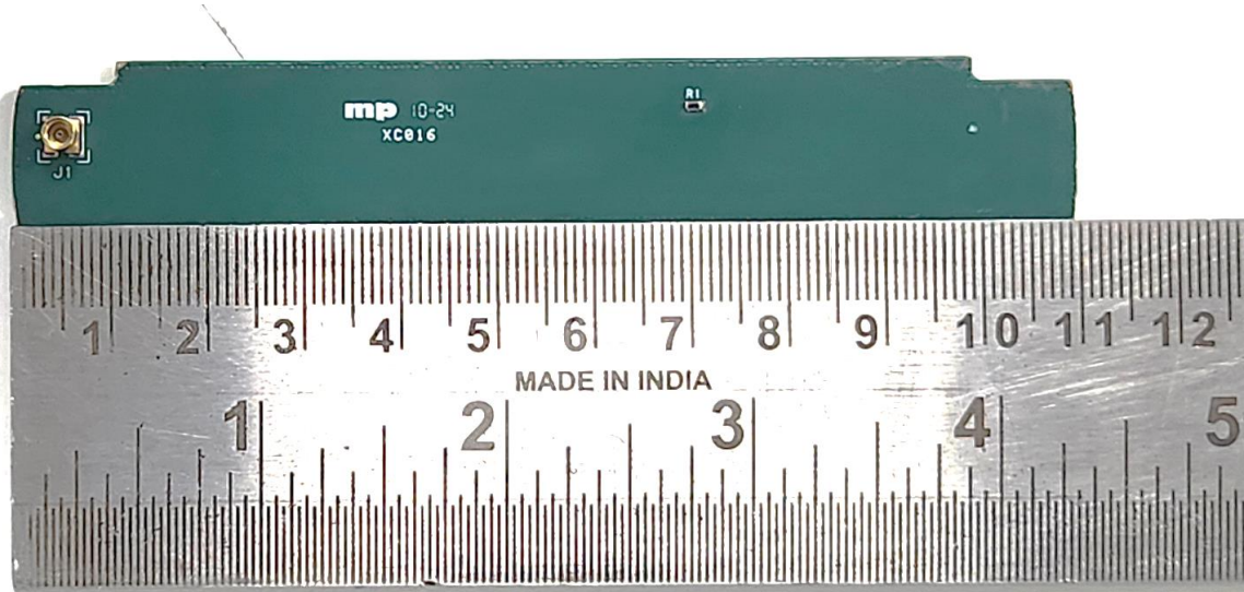
RFID Coupler – LUPUS14V2 (Rear Side)
