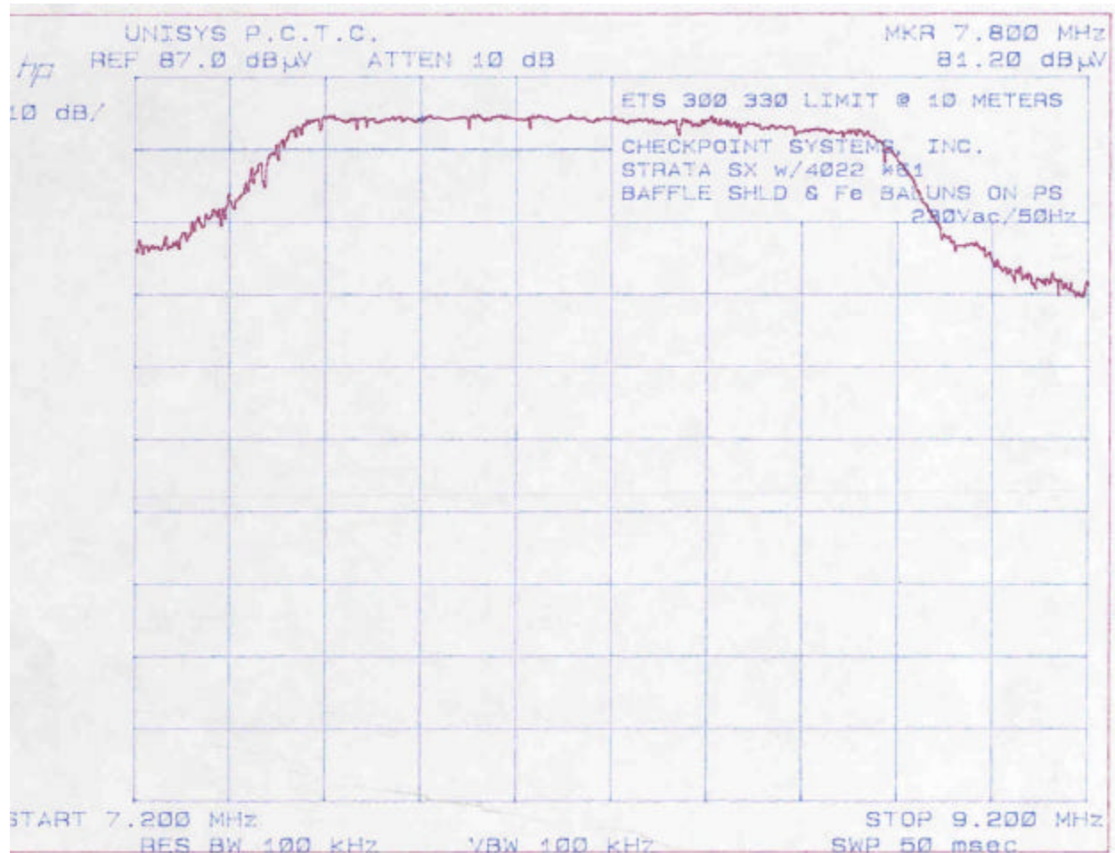
Photo 5 – Bandwidth Plot
