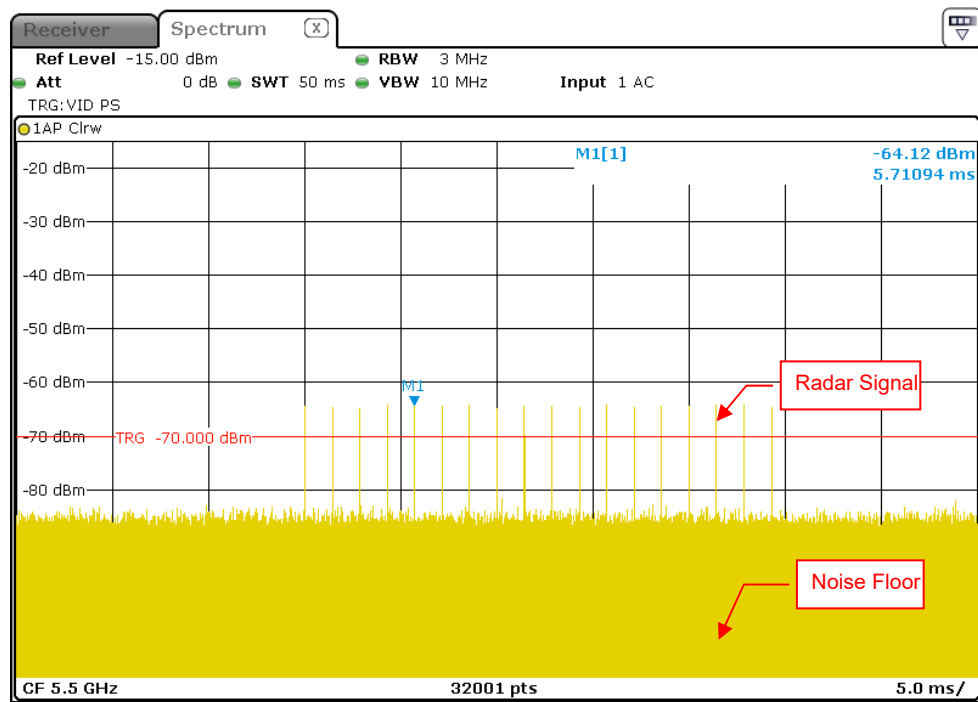
Radar Signal 0
