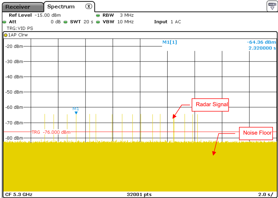
Radar Signal 5
