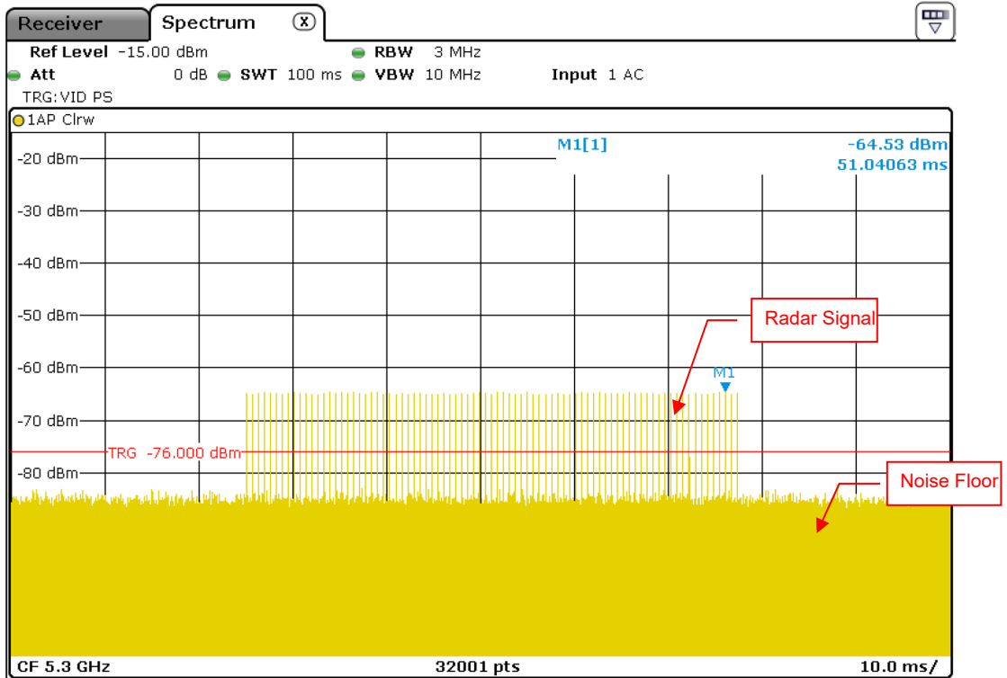
Radar Signal 1
