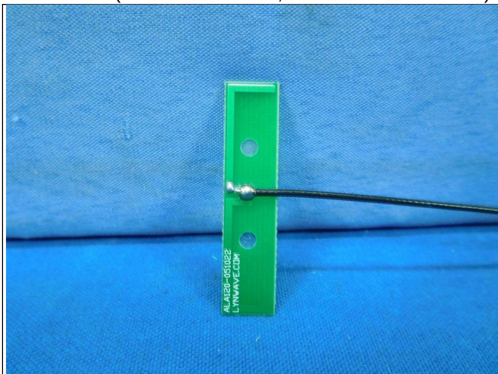
Antenna 28 (Brand: LYNWAVE ; Model: ALA120-051022)
