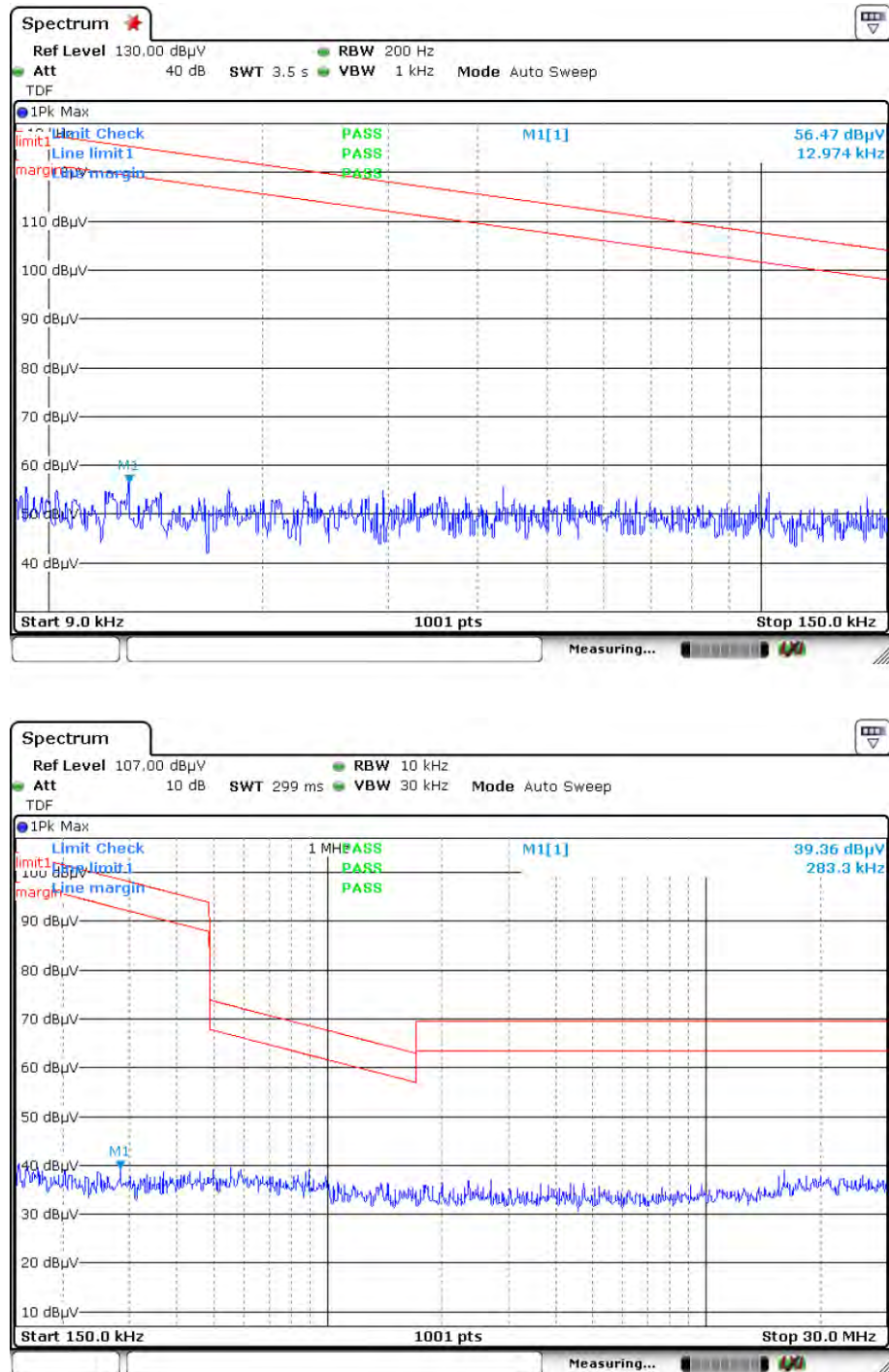
Figure 4: Test figure of Radiated Spurious Emissions (9kHz – 30MHz), 802.11b, (Mid)
