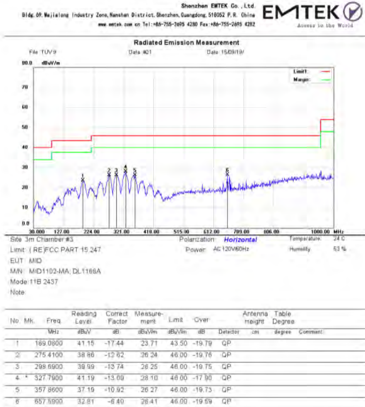
Figure 5: Test figure of Radiated Spurious Emissions (30MHz – 1GHz), 802.11b, (Mid)
