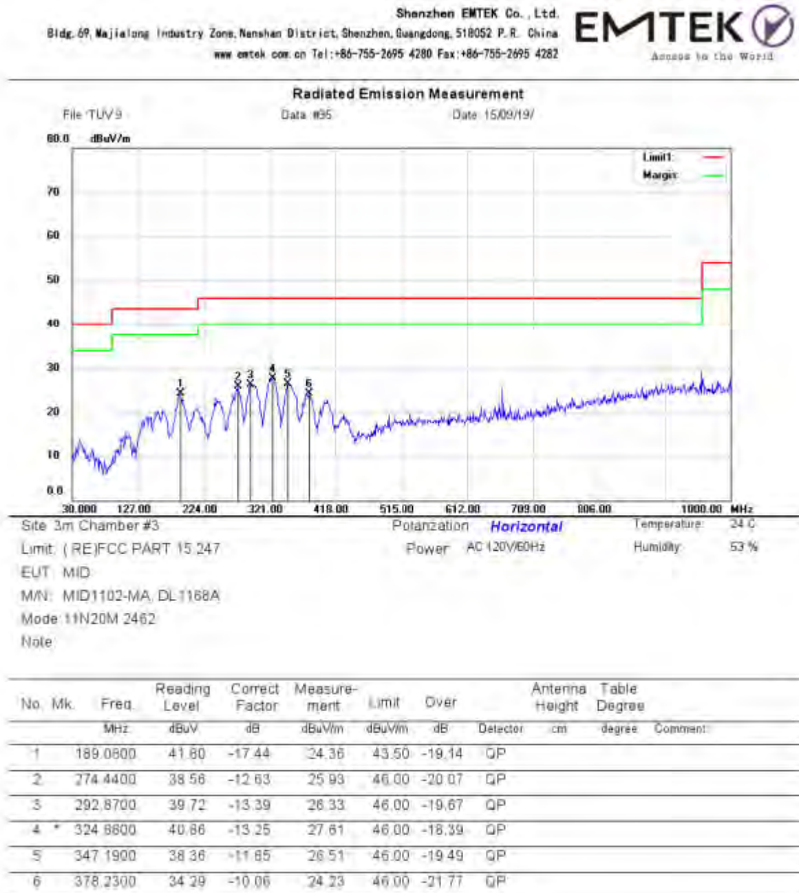
Figure 20: Test figure of Radiated Spurious Emissions (30MHz – 1GHz), 802.11n(HT20), (High)
