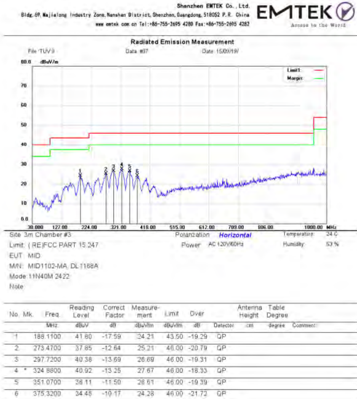
Figure 22: Test figure of Radiated Spurious Emissions (30MHz – 1GHz), 802.11n(HT40), (Low)
