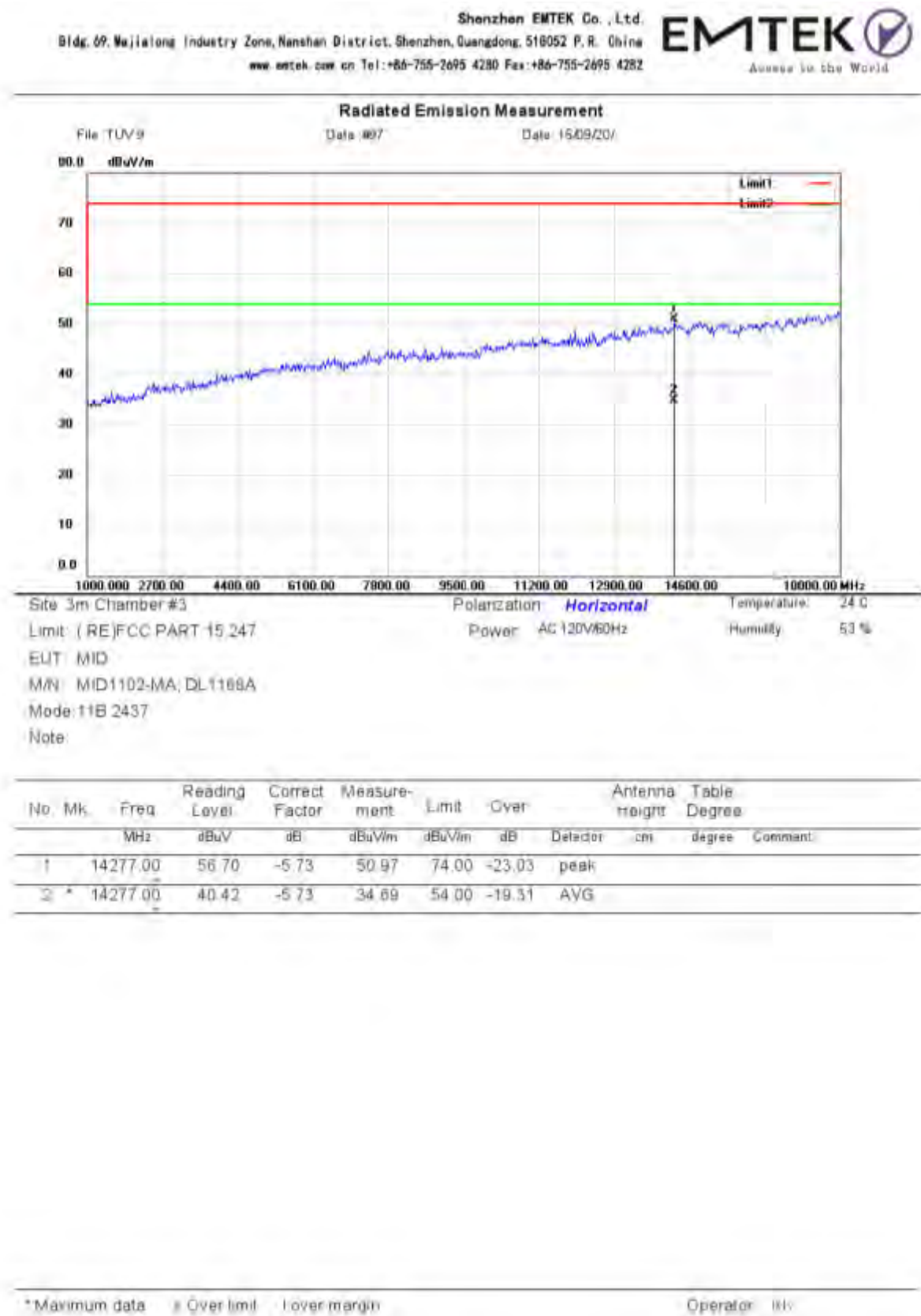
Figure 6: Test figure of Radiated Spurious Emissions (1GHz –25GHz), 802.11b, (Mid)
