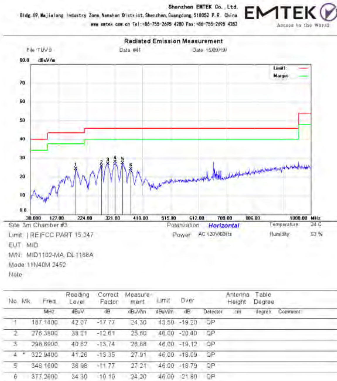
Figure 26: Test figure of Radiated Spurious Emissions (30MHz – 1GHz), 802.11n(HT40), (High)
