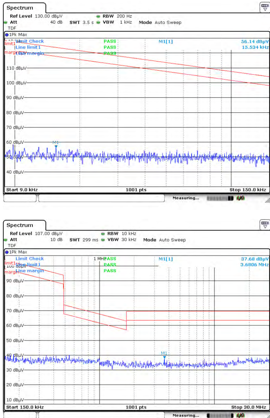
Figure 7: Test figure of Radiated Spurious Emissions (9kHz – 30MHz), 802.11b, (High)
