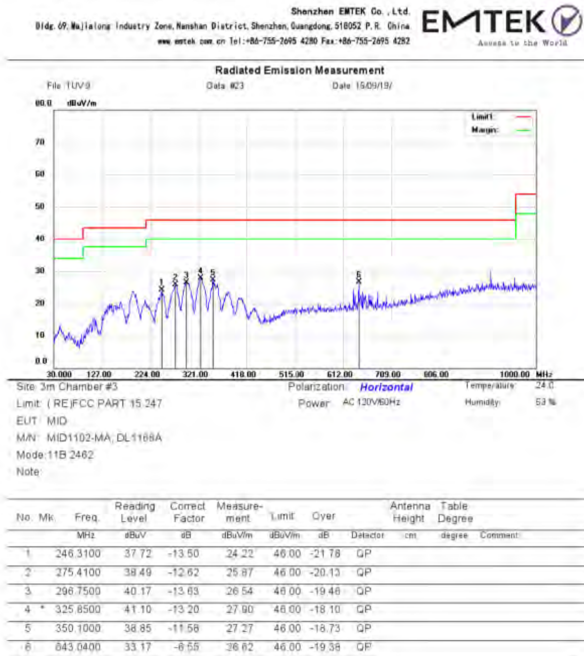
Figure 8: Test figure of Radiated Spurious Emissions (30MHz – 1GHz), 802.11b, (High)
