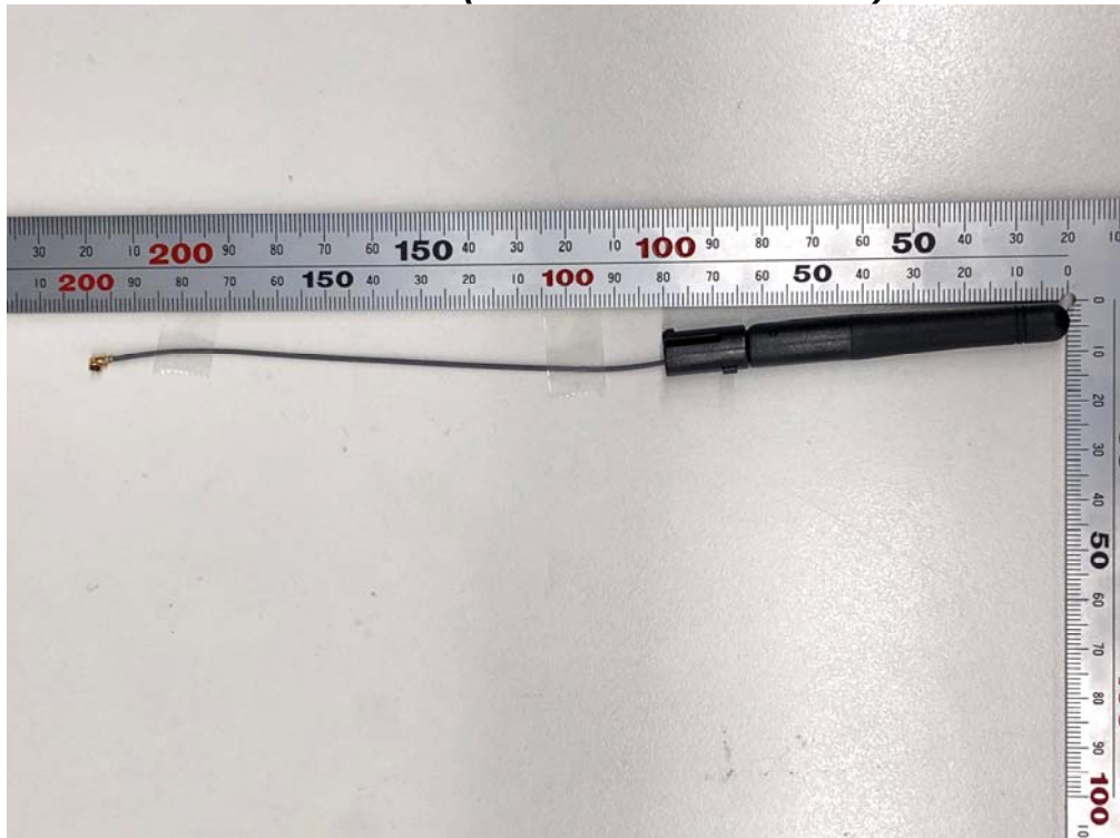
Antenna – 2 (Part No.: ANTDC-081A0)
