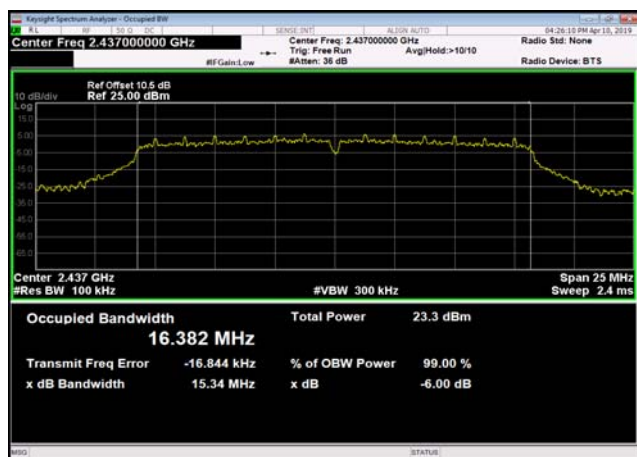
6dB Bandwidth-802.11g,2437MHz
