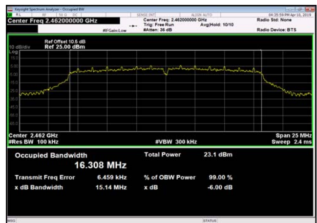
6dB Bandwidth-802.11g,2462MHz
