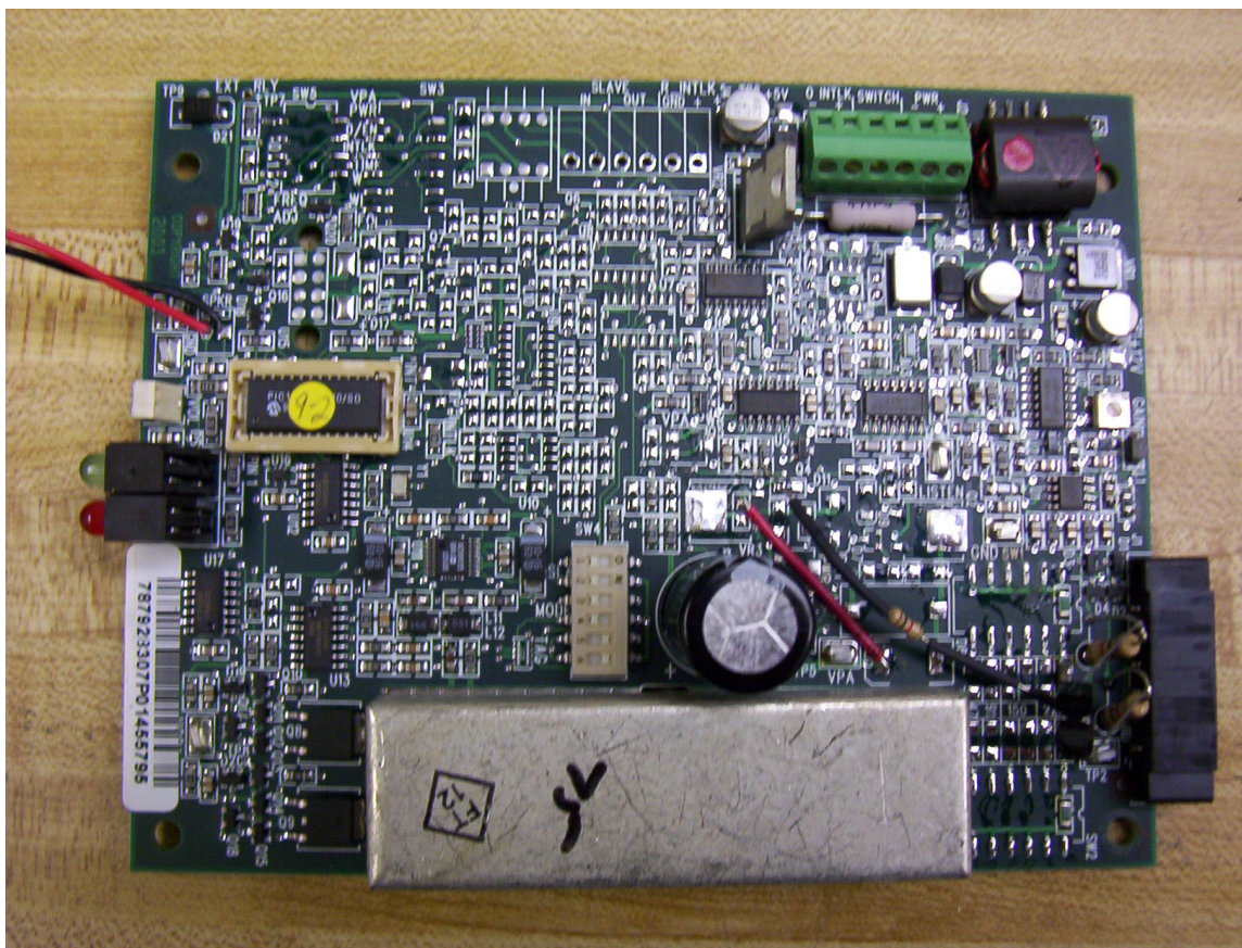
Checkpoint Systems, Inc.: Internal Photo of Component side of CP9-2 PCB
