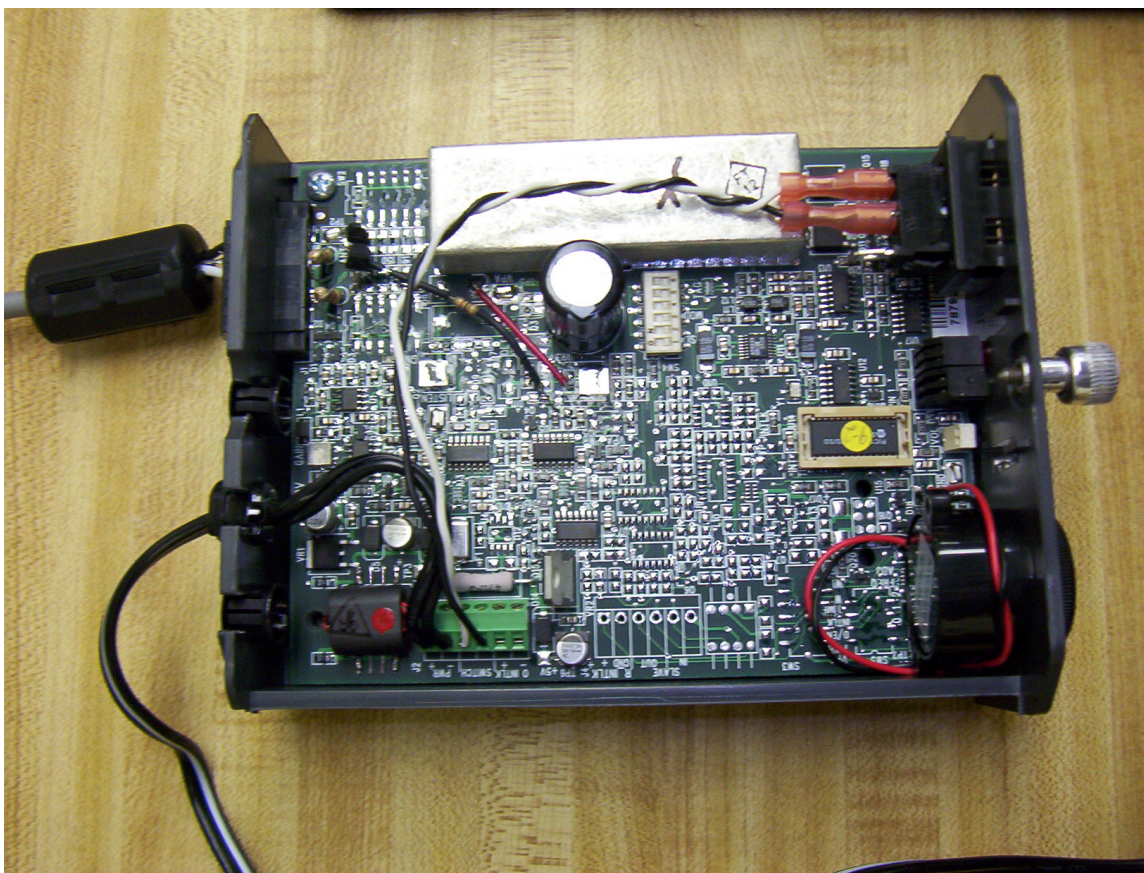
Checkpoint Systems, Inc.: Internal Photo of CP9-2 with cover removed
