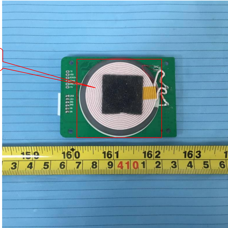
Wireless Charger Antenna
