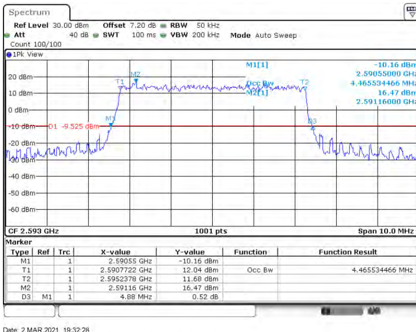
Band41-5MHz-QPSK-40620-25RB#0-4.466
