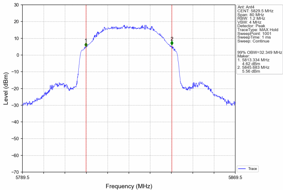
40M_HCH_5829.5MHz_Ant4_NTNV
