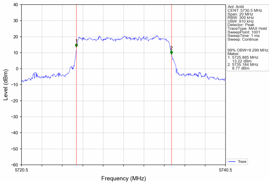
10M_LCH_5730.5MHz_Ant4_NTNV
