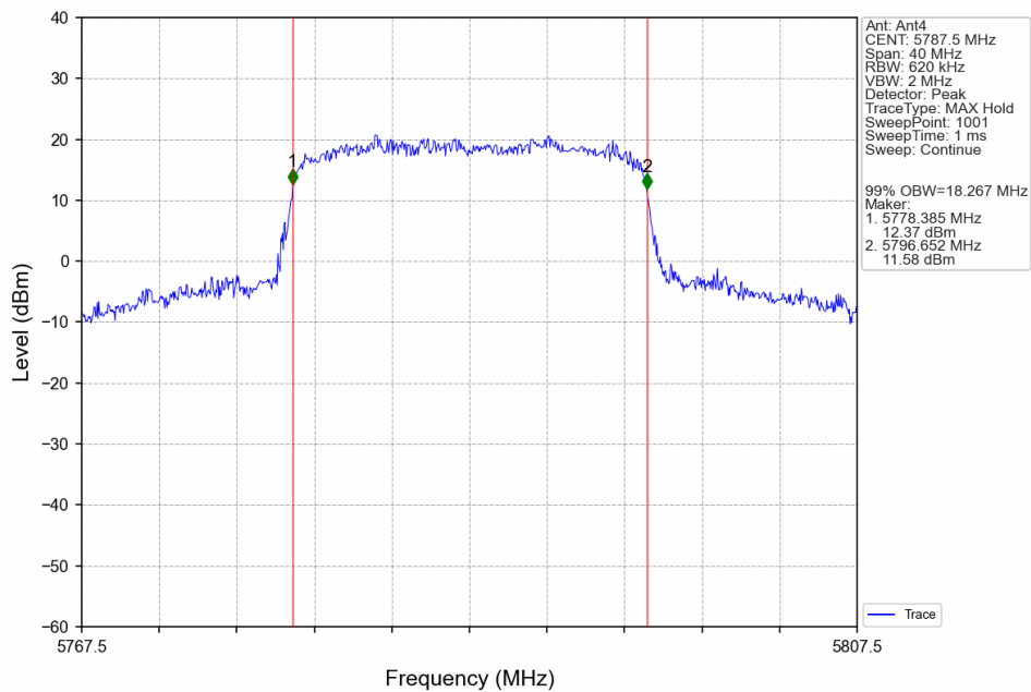
20M_MCH_5787.5MHz_Ant4_NTNV
