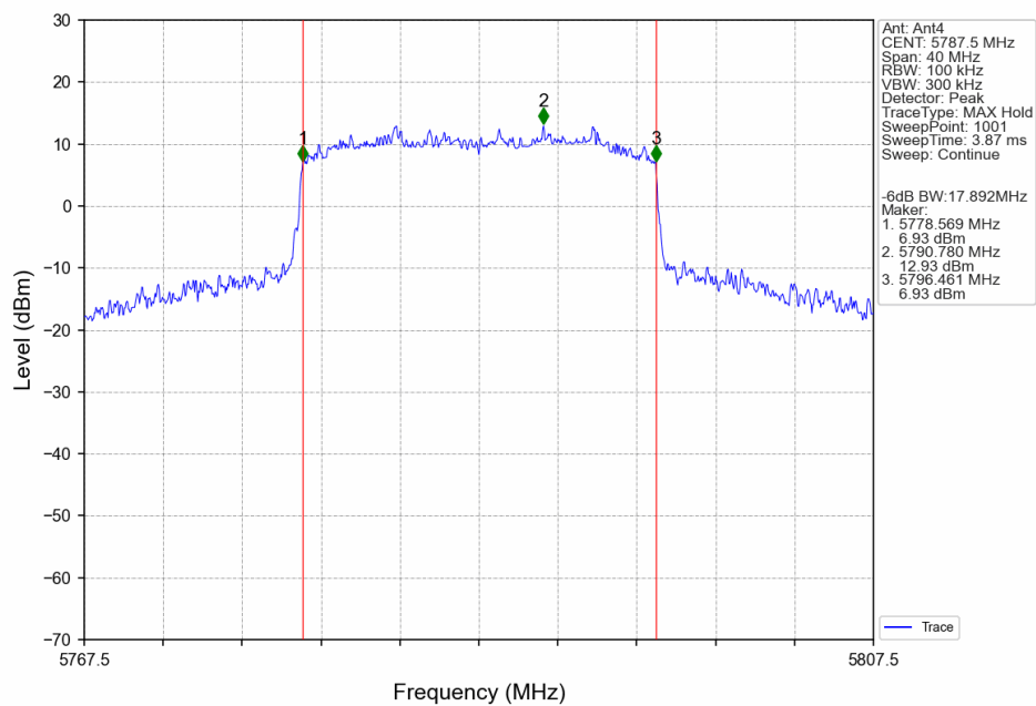
20M_MCH_5787.5MHz_Ant4_NTNV
