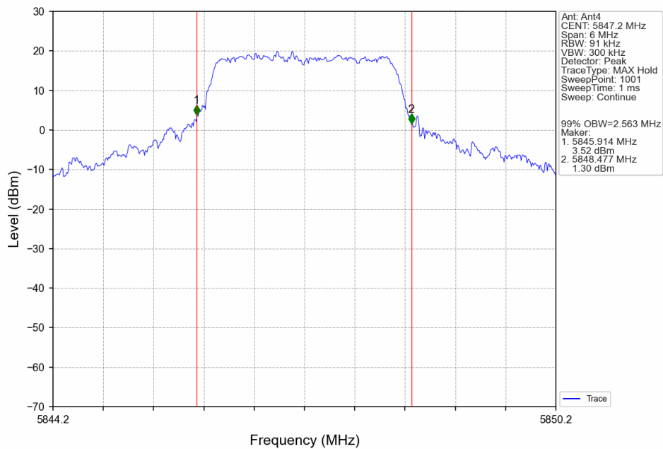
3M_HCH_5847.2MHz_Ant4_NTNV
