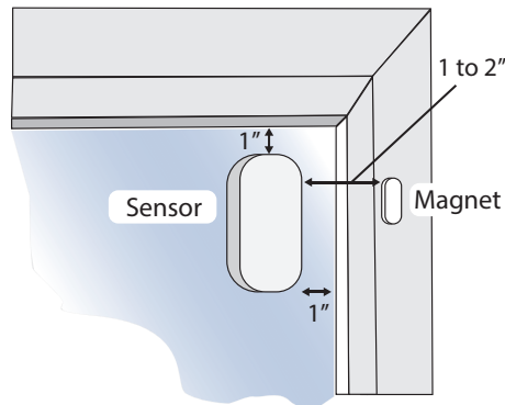
Figure 3. Standard Glass Mounting
