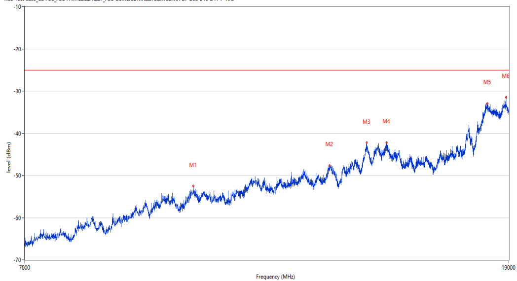
RSE Test case_FCC_FCC PART22&24&27_FCC GSM&CDMA&LTE&WCDMA B7 B38 B40 B41 7-19G
