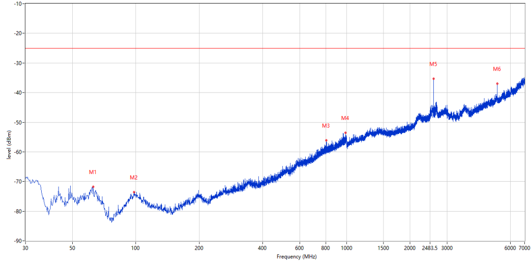
RSE Test case FCC_FCC PART22&24&27_FCC LTE B38
