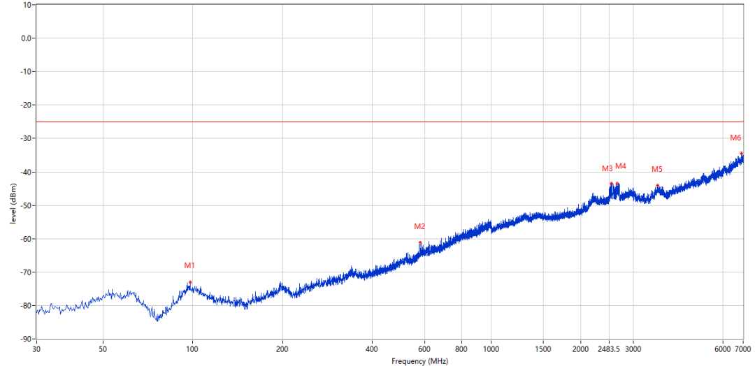
RSE Test case_CE_FCC_FCC PART22&24&27_FCC PART 27_2535_LTE B7
