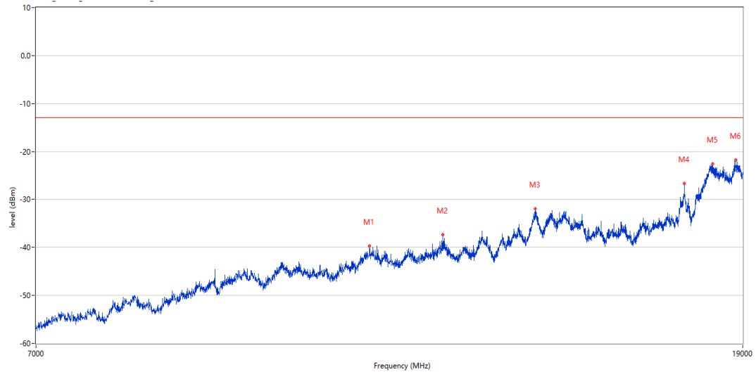
RSE Test case_FCC_FCC PART22&24&27_FCC GSM&CDMA&LTE&WCDMA 7-19G
