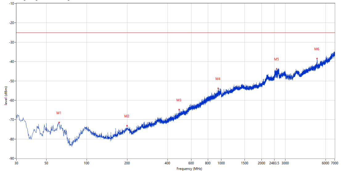
RSE Test case_CE FCC_FCC PART22&24&27_FCC LTE B38
