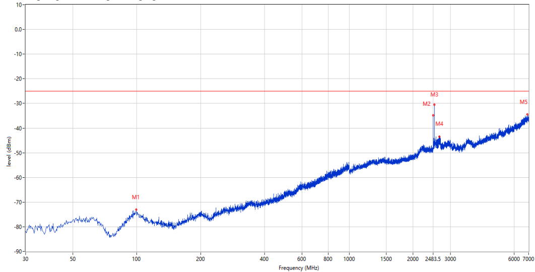
RSE Test case FCC_FCC PART22&24&27_FCC PART 27_2535_LTE B7
