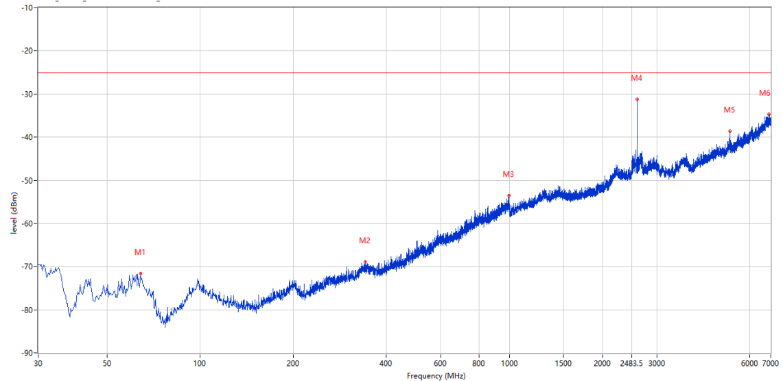
RSE Test case_CE_FCC_FCC PART22&24&27_FCC LTE B38
