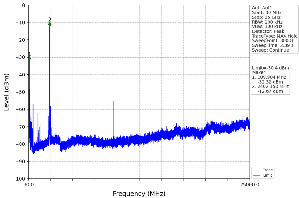
GFSK_DH5_LCH_2402MHz_Ant1_NTNV
