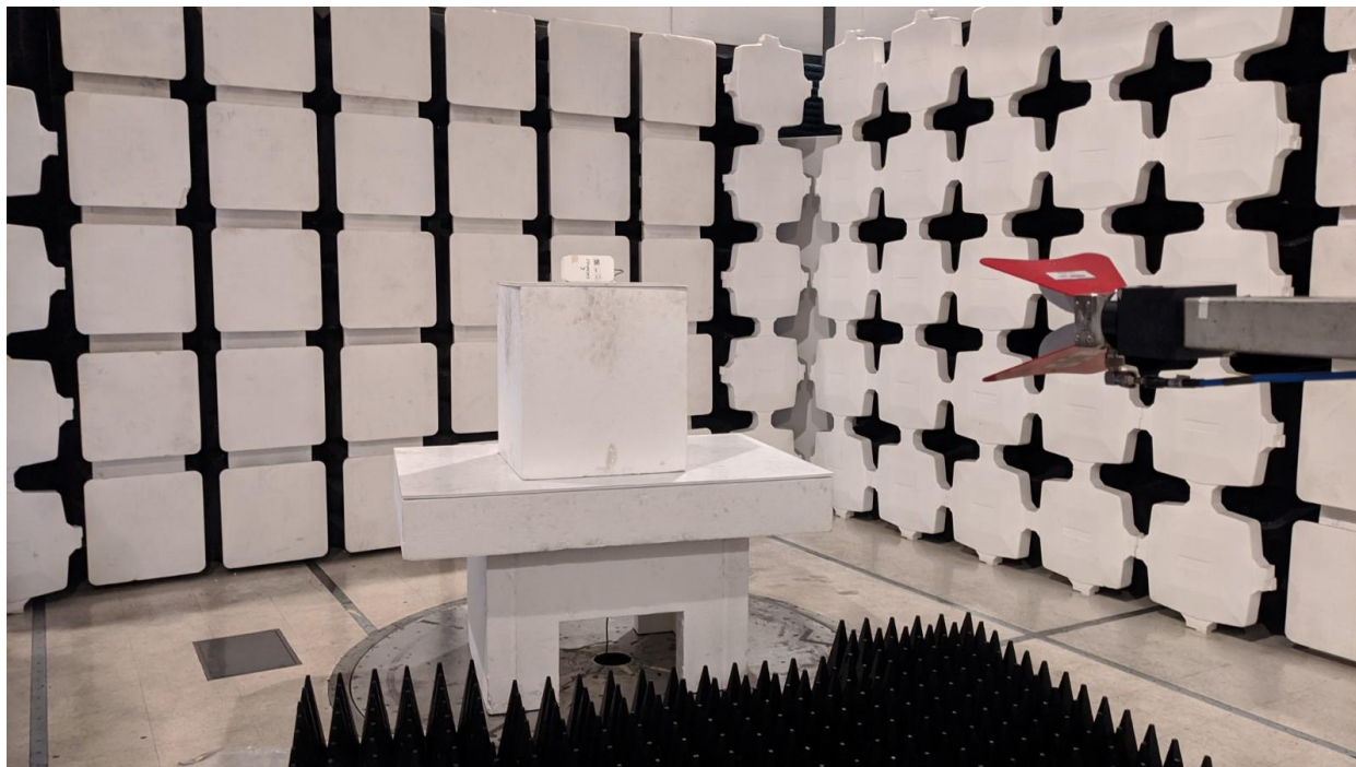
Radiated RF 1 - 18GHz
