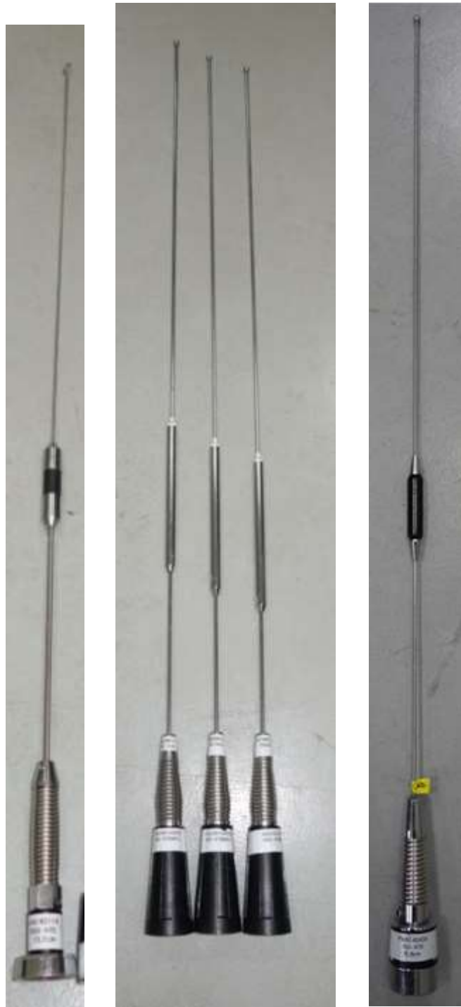
UHF2 Antenna kit numbers, from left to right HAE4011A, *RAE4014ARB (3pcs), PMAE4043A
