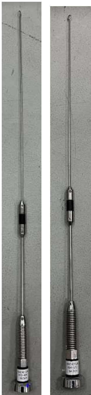
UHF2 Antenna kit numbers, from left to right HAE4012A, HAE4013A
