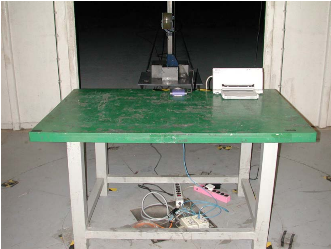
Front View of Radiated Test (Mode 1-Horn)
