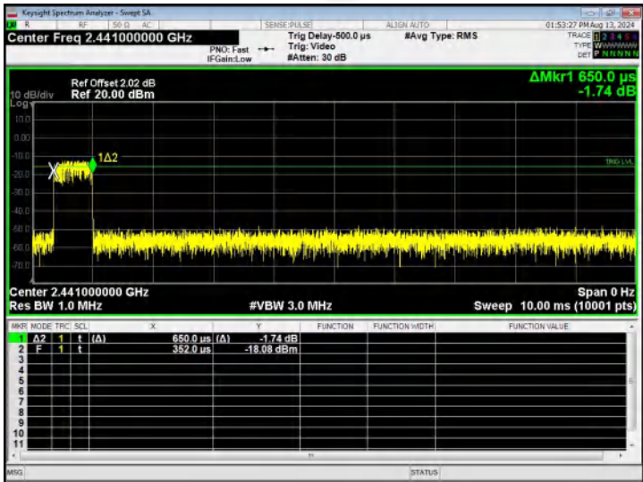
8-DPSK 3DH3 2441MHz
