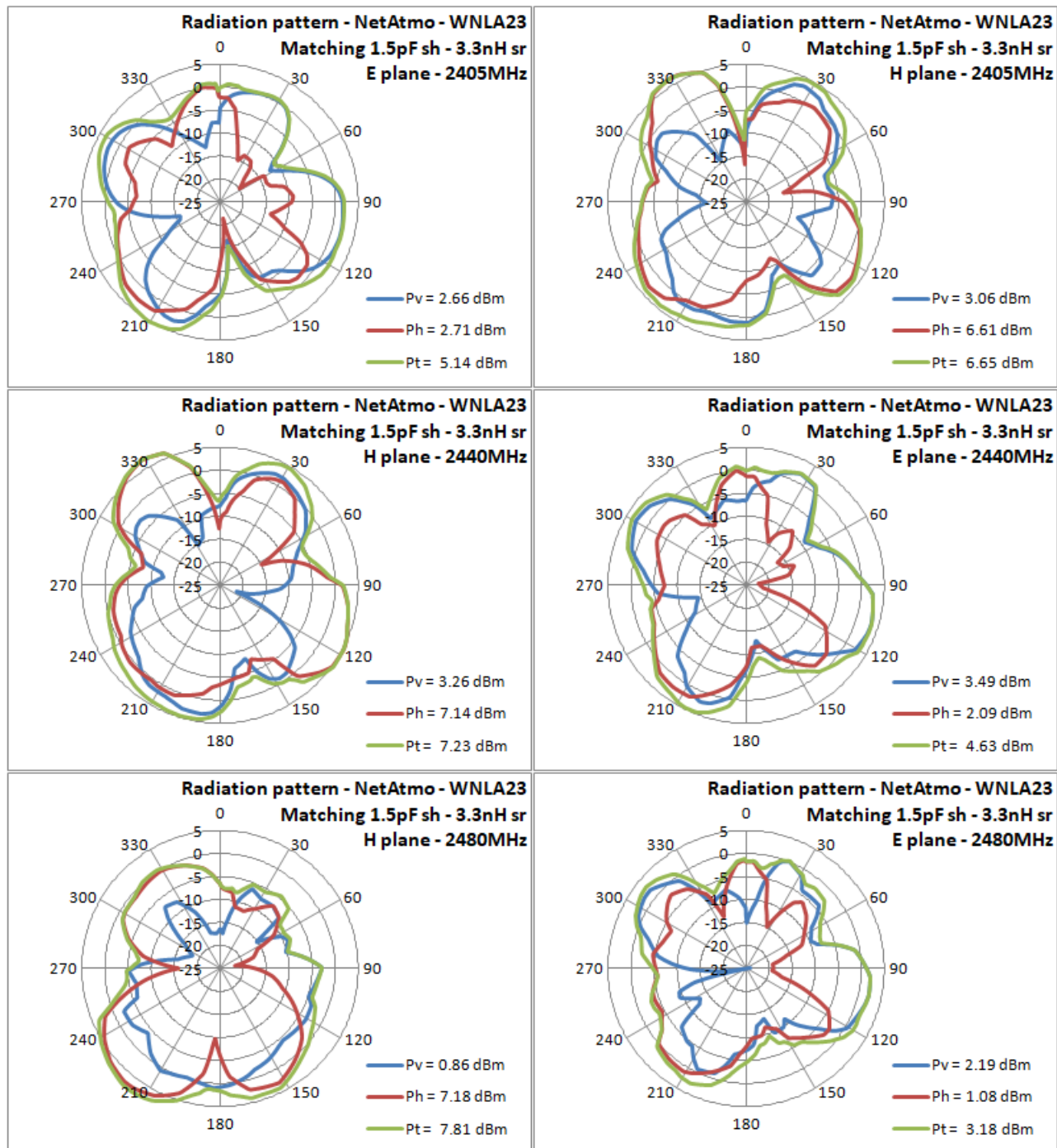
figure 17. From left to right, from top to bottom, Radiation pattern for H & E planes for the 2405, 2440 & 2480MHz frequencies for WNLA23 with proposed matching network
