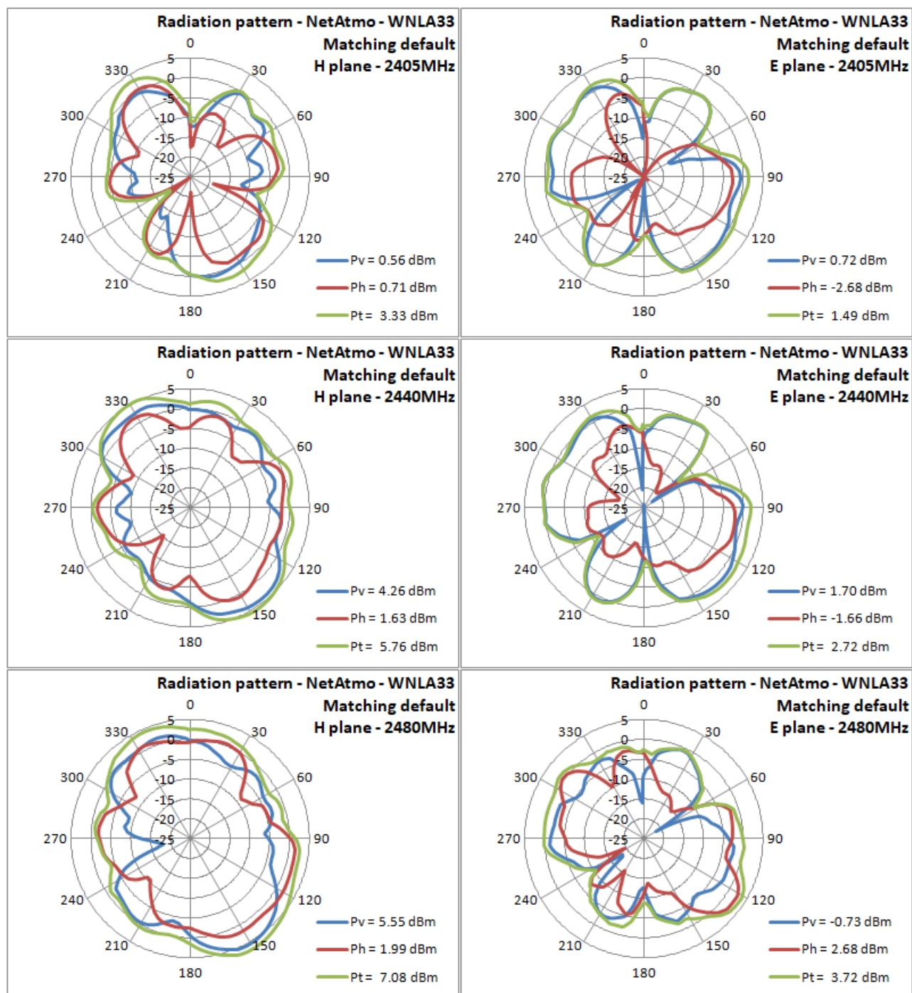
figure 20. From left to right, from top to bottom, Radiation pattern for H & E planes for the 2405, 2440 & 2480MHz frequencies for WNLA33 with default matching network
