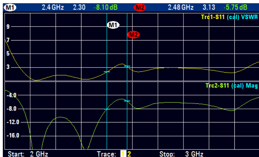
figure 4. WNAL63 antenna matching with the default matching Network
