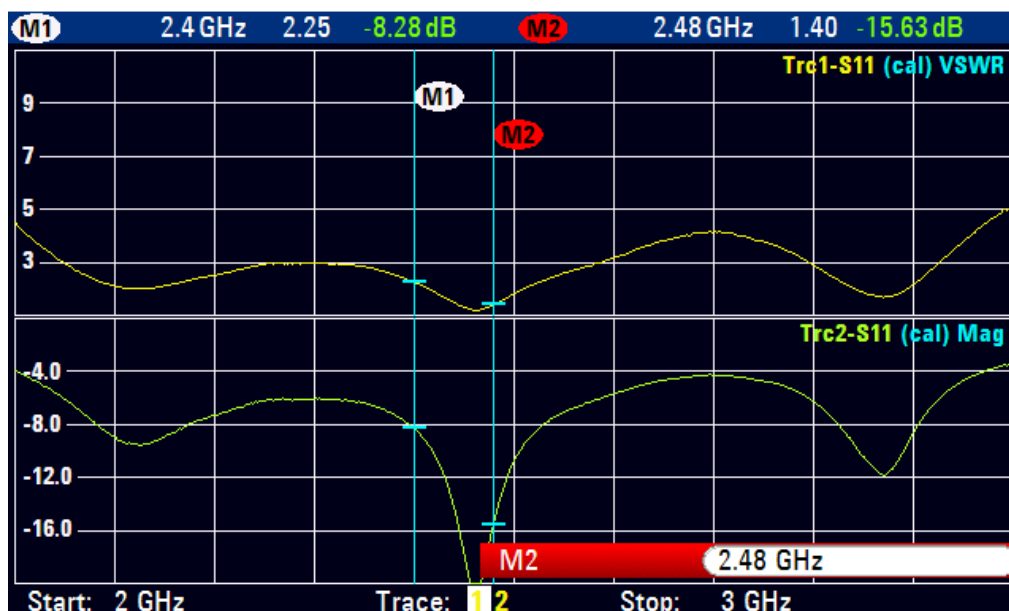
figure 5. WNAL33 antenna matching with the default matching Network
