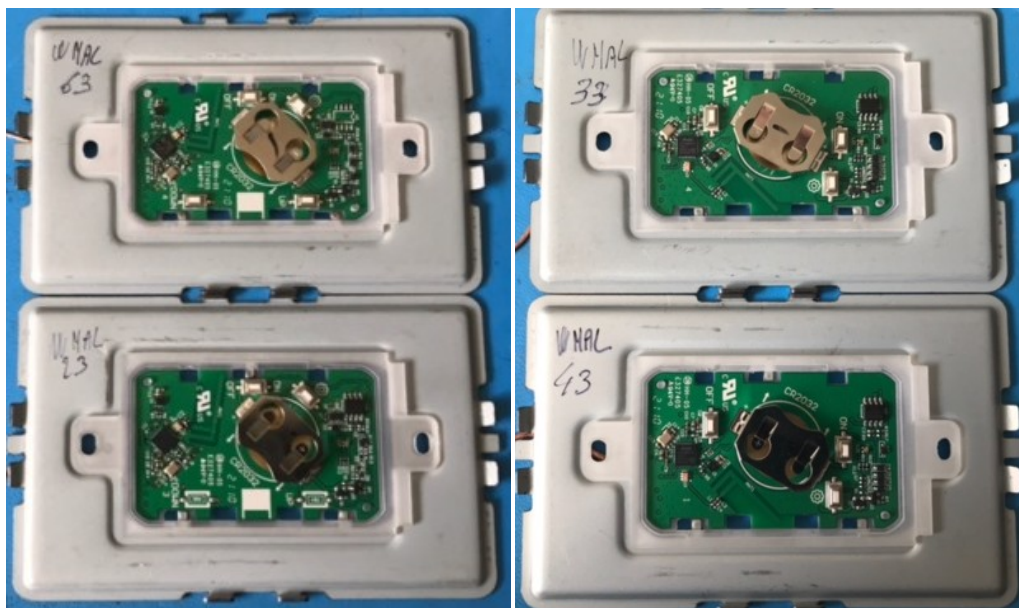
figure 1. From top to bottom and left to right, WNAL 63, WNAL23, WNAL33 & WNAL43
