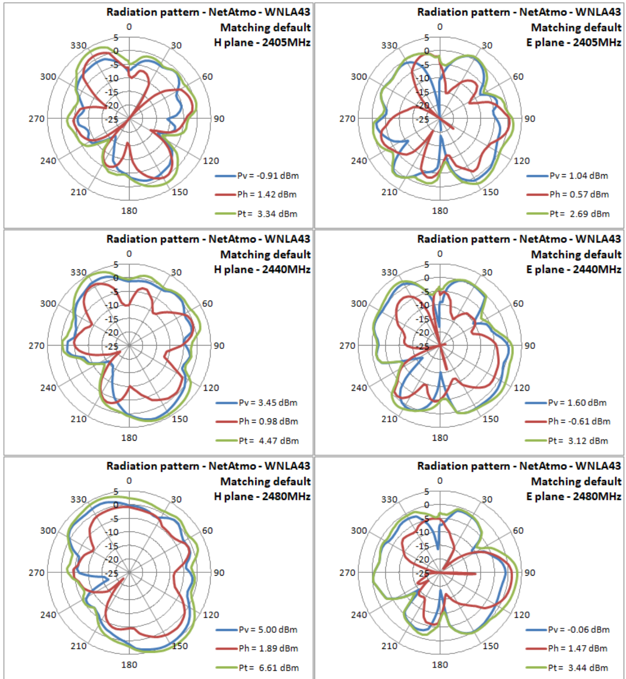
figure 18. From left to right, from top to bottom, Radiation pattern for H & E planes for the 2405, 2440 & 2480MHz frequencies for WNLA43 with default matching network
