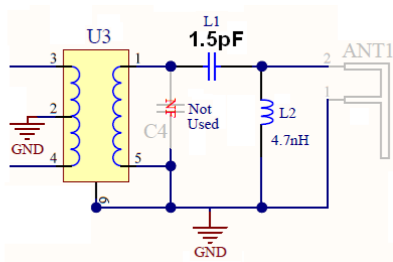
figure 10. antenna matching circuit proposed for WNAL33 & WNAL43 product: "Ant-4.7nH shunt – 1.5pF serie"
