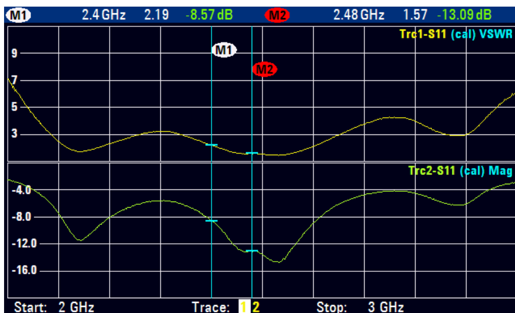
figure 6. WNAL43 antenna matching with the default matching Network
