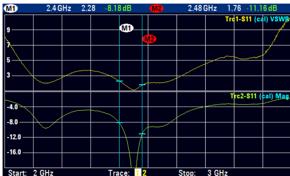
figure 8. Frequency response of the WNAL23 antenna with the matching network proposed : "Ant-1.5pf shunt – 3.3nH serie"
