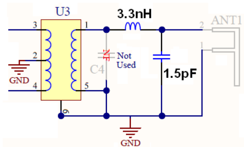
figure 7. antenna matching circuit proposed for WNAL23 & WNAL63 product: "Ant-1.5pf shunt – 3.3nH serie"
