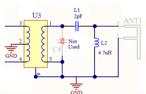
figure 2. Matching Network used by default for all products
