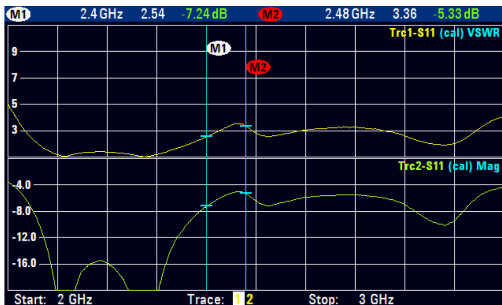
figure 3. WNAL23 antenna matching with the default matching Network
