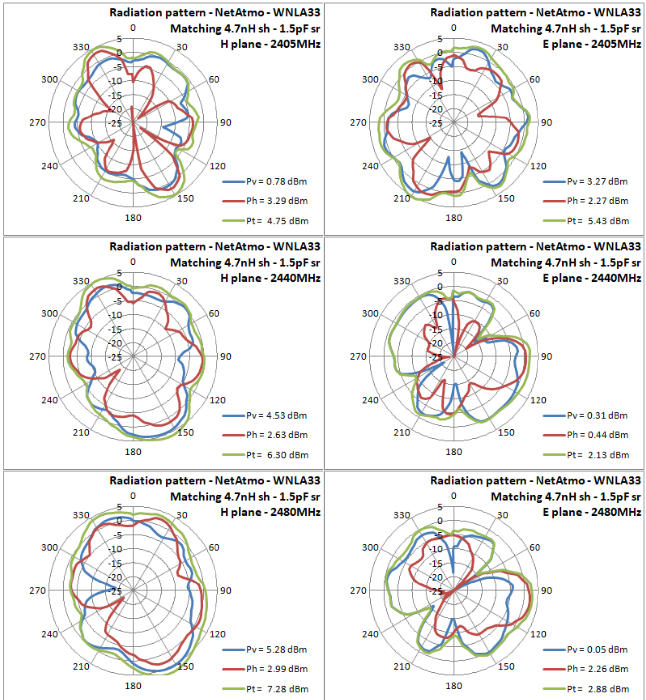
figure 21. From left to right, from top to bottom, Radiation pattern for H & E planes for the 2405, 2440 & 2480MHz frequencies for WNLA33 with proposed matching network
