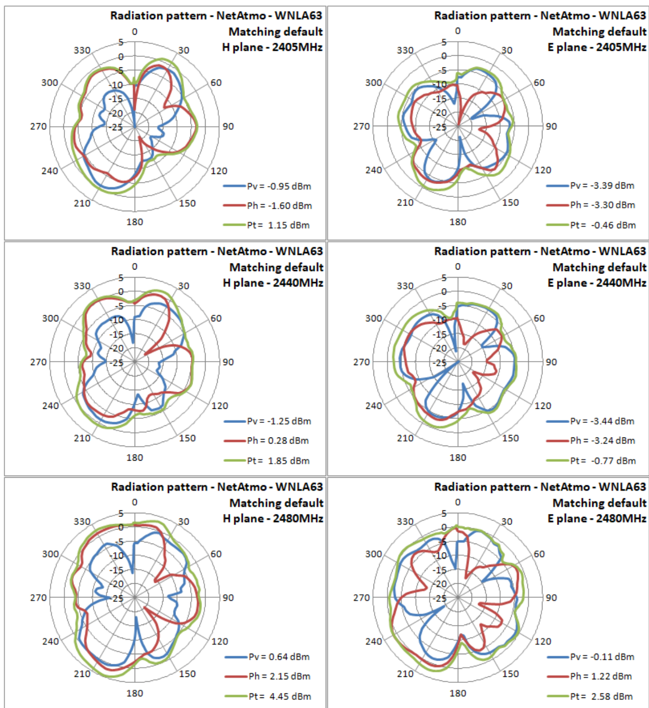
figure 14. From left to right, from top to bottom, Radiation pattern for H & E planes for the 2405, 2440 & 2480MHz frequencies for WNLA63 with default matching network
