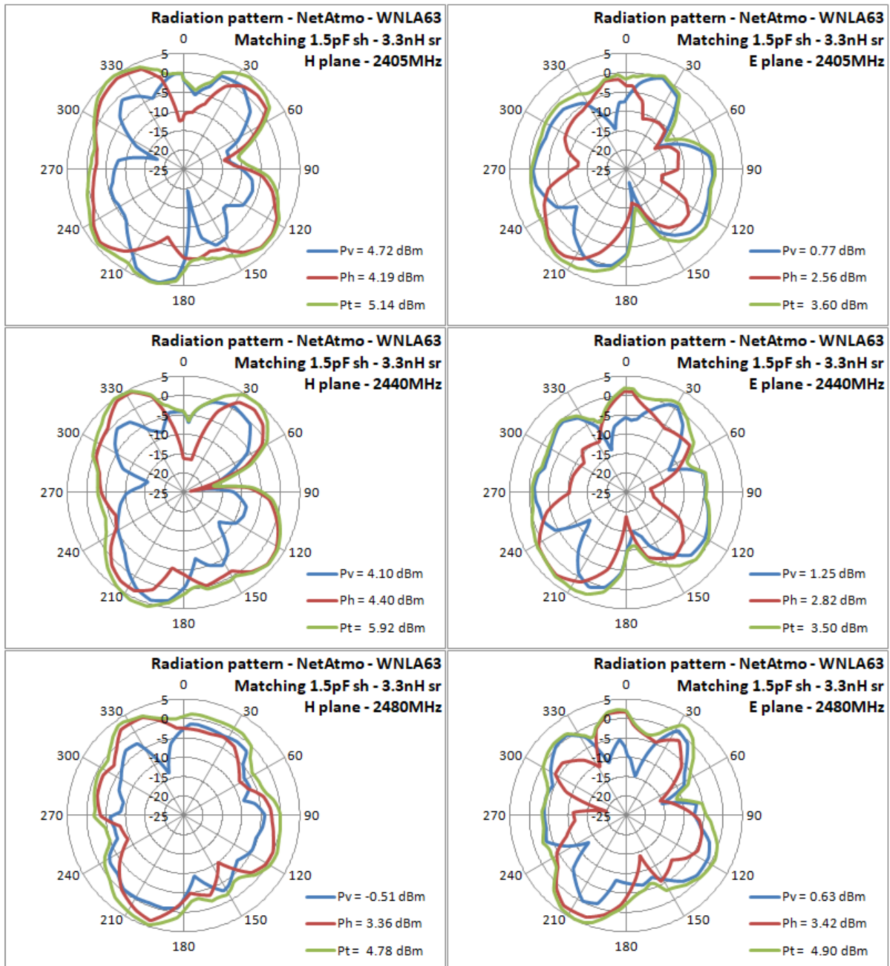
figure 15. From left to right, from top to bottom, Radiation pattern for H & E planes for the 2405, 2440 & 2480MHz frequencies for WNLA63 with proposed matching network
