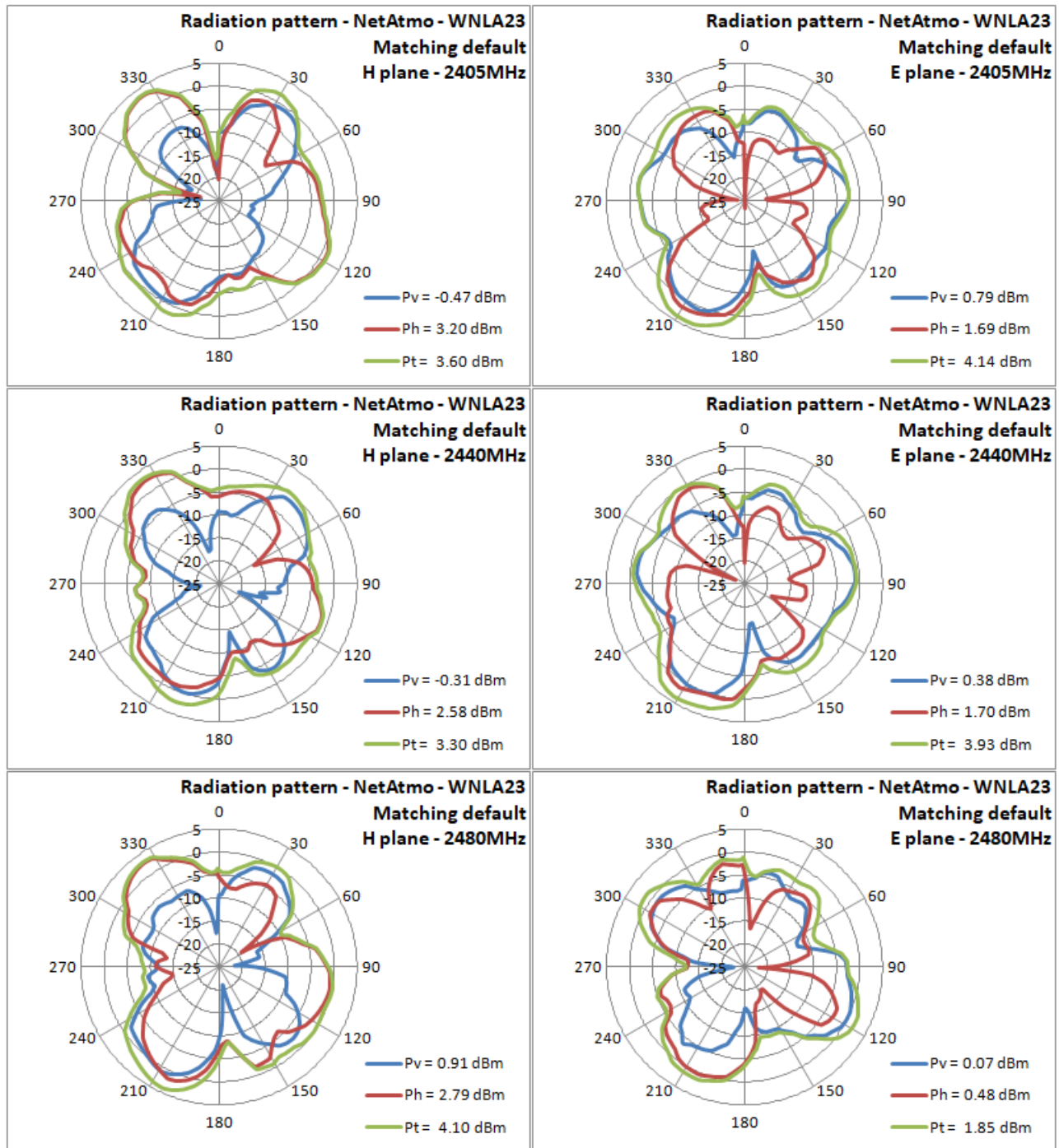
figure 16. From left to right, from top to bottom, Radiation pattern for H & E planes for the 2405, 2440 & 2480MHz frequencies for WNLA23 with default matching network
