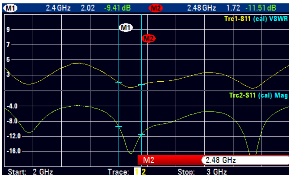
figure 11. Frequency response of the WNAL23 antenna with the matching network proposed : "Ant-4.7nH shunt – 1.5pF serie"
