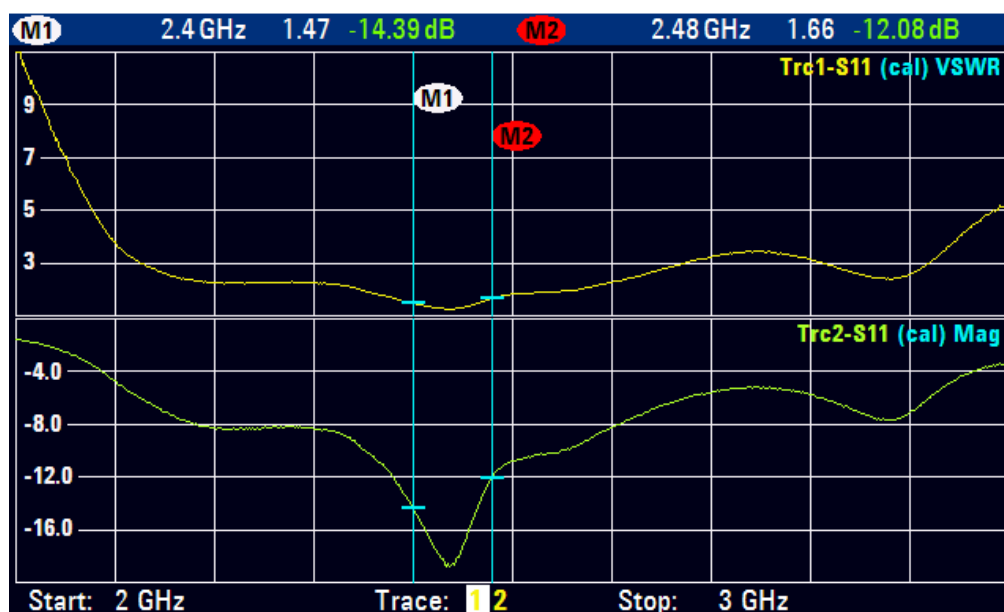
figure 9. Frequency response of the WNAL63 antenna with the matching network proposed : "Ant-1.5pF shunt – 3.3nH seriee"
