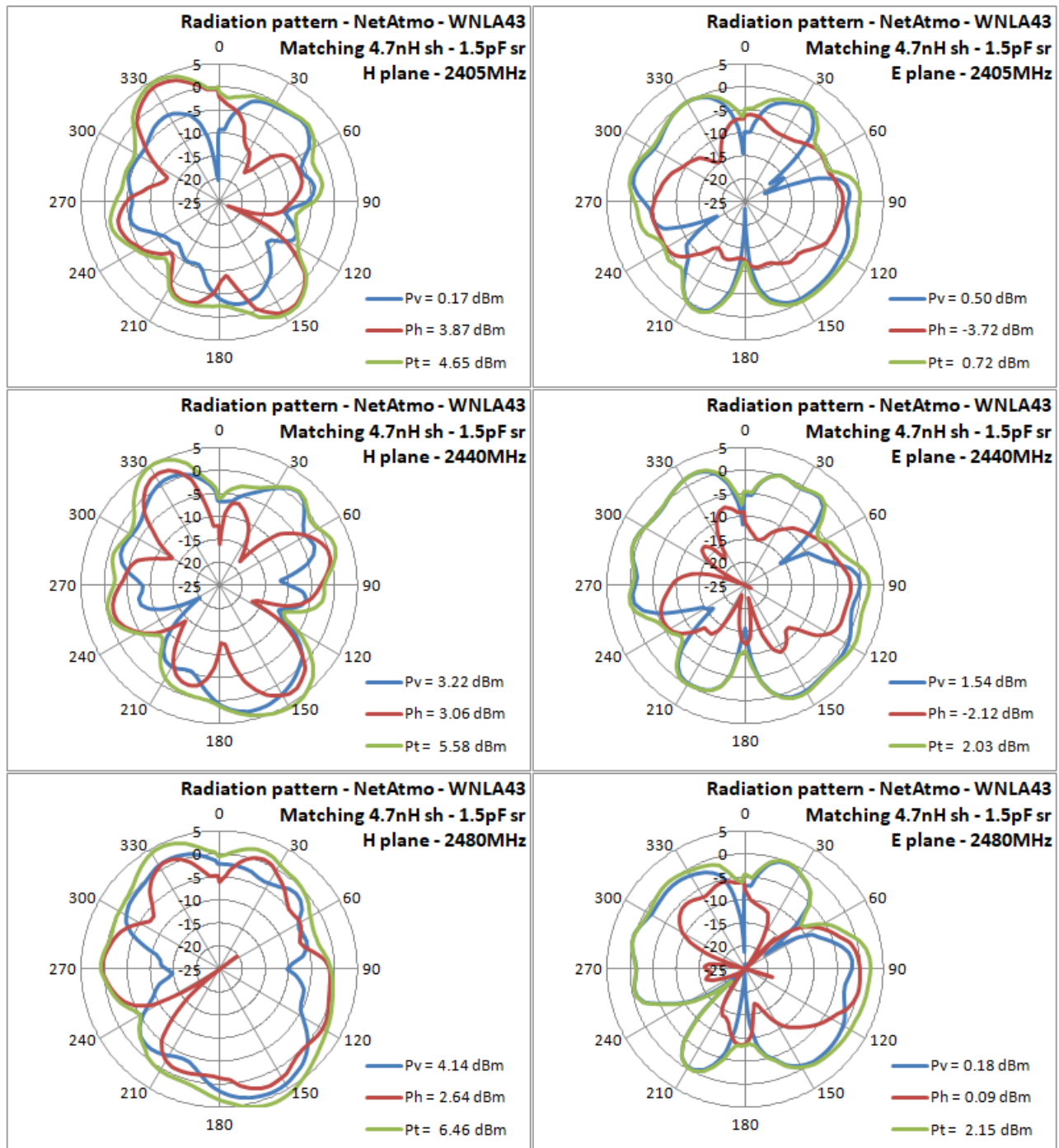
figure 19. From left to right, from top to bottom, Radiation pattern for H & E planes for the 2405, 2440 & 2480MHz frequencies for WNLA43 with proposed matching network
