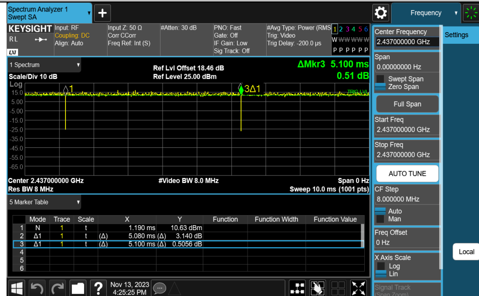
NTNV-11N20SISO-Ant1-2437
