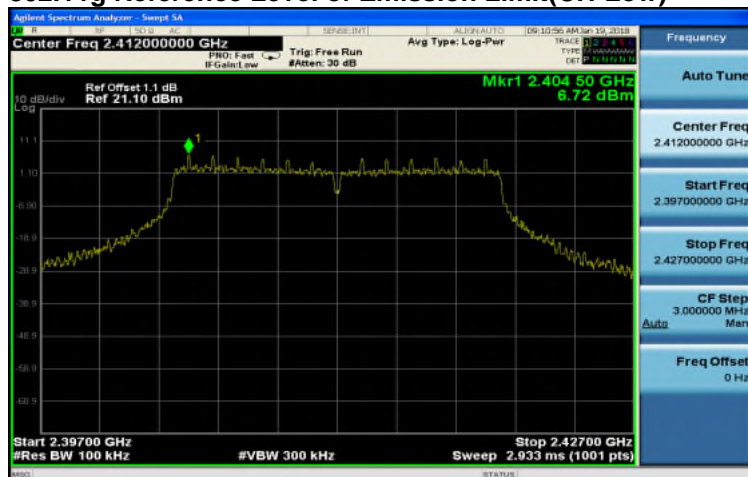
802.11g Reference Level of Emission Limit (CH-Low)
