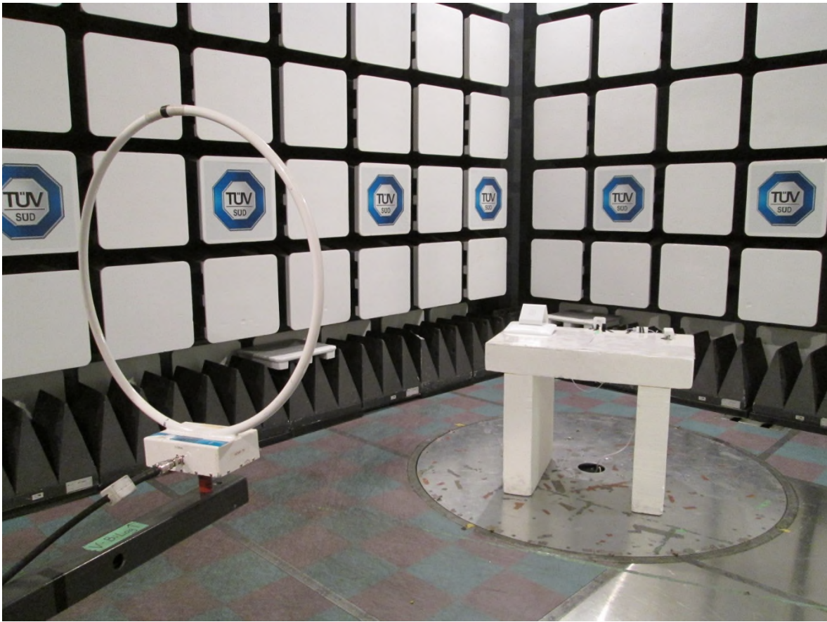
NFC Test setup photo 1 Radiated measurements, 9 kHz – 30 MHz
