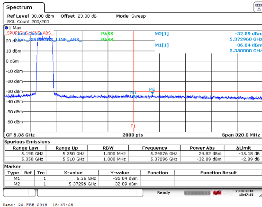
Figure 9 Spurious Emissions (Upper Band Edge) – 256QAM (5240.0 MHz) (20MHz Channel BW)
