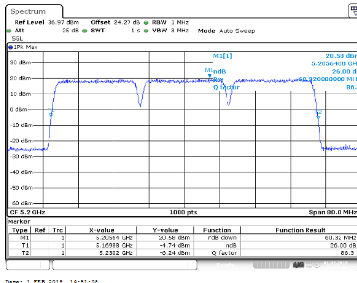
Figure 82 Occupied Bandwidth – 64QAM (5180/ 5200/5220 MHz) (2 X 20MHz Channel BW)
