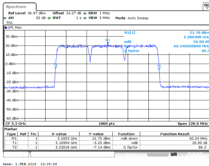
Figure 79 Occupied Bandwidth – 16QAM (5180/ 5200/5220 MHz) (2 X 20MHz Channel BW)
