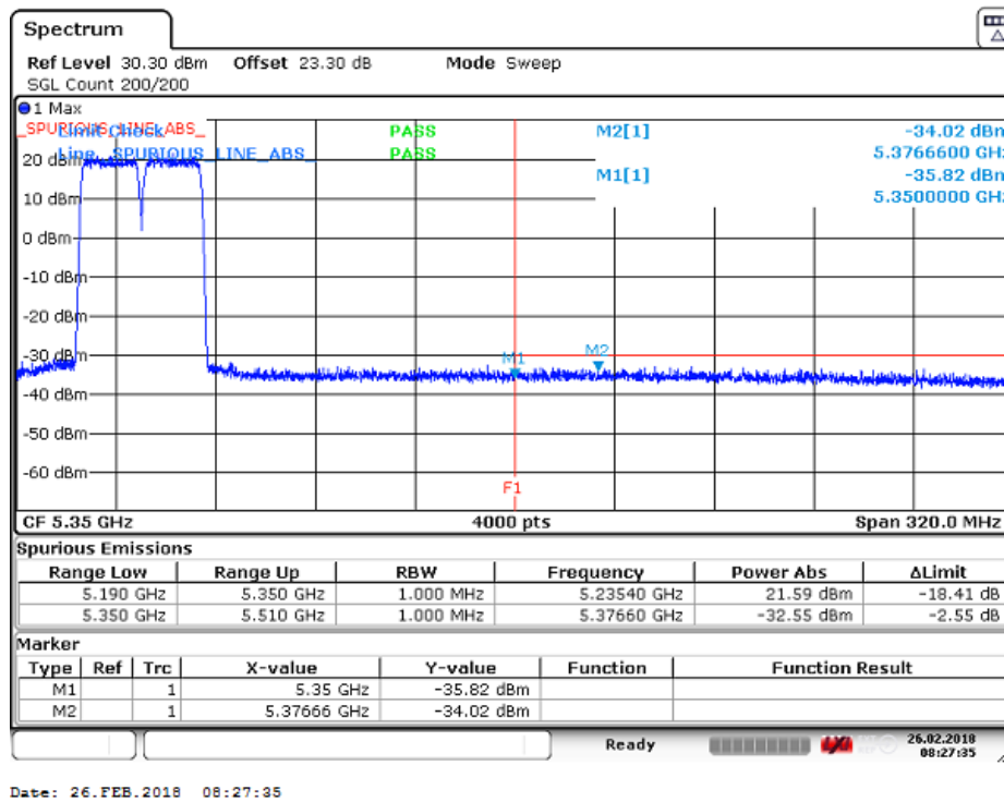
Figure 117 Spurious Emissions (Upper Band Edge) – 64QAM (5220.0/ 5240.0 MHz) (2 X 20MHz Channel BW)
