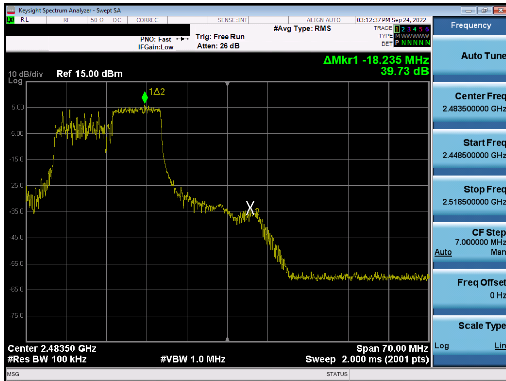
Plot 7-42. Band Edge Plot MIMO ANT1 (802.11ax OFDMA – 106 Tones – Ch. 11)
