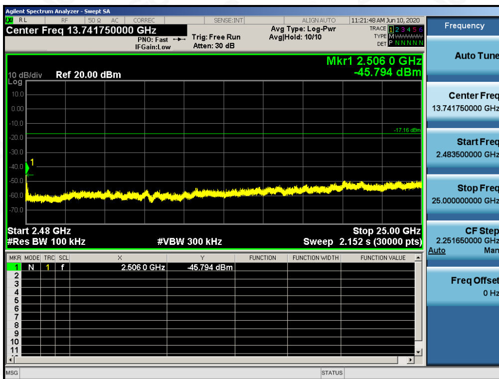
TEST PLOT OF OUT OF BAND EMISSIONS OF 8DPSK MODULATION IN MIDDLE CHANNEL
