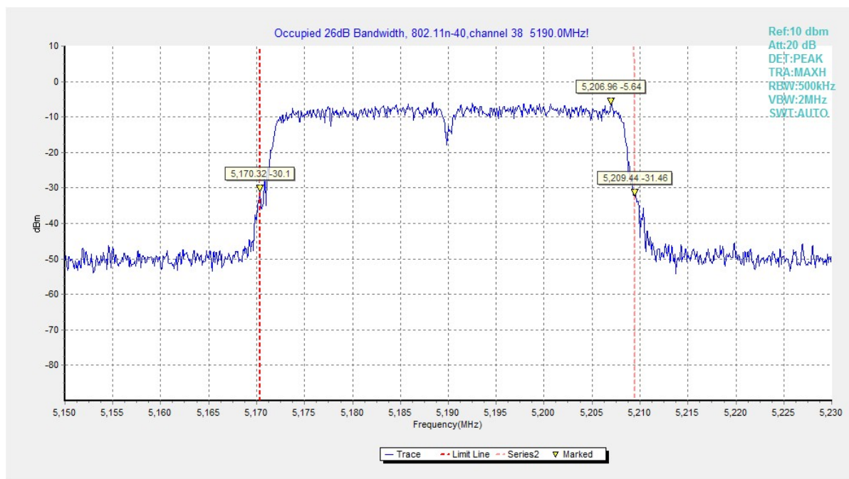
Fig. 28 Occupied 26dB Bandwidth (802.11n40, 5190MHz)
