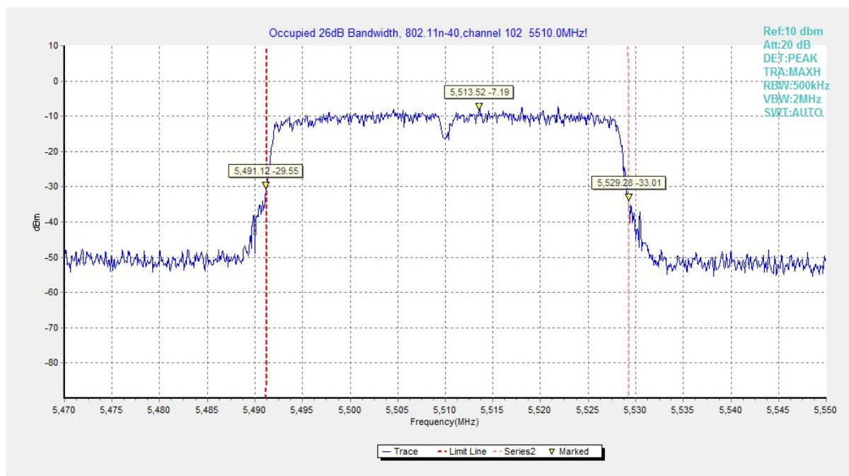
Fig. 32 Occupied 26dB Bandwidth (802.11n40, 5510MHz)
