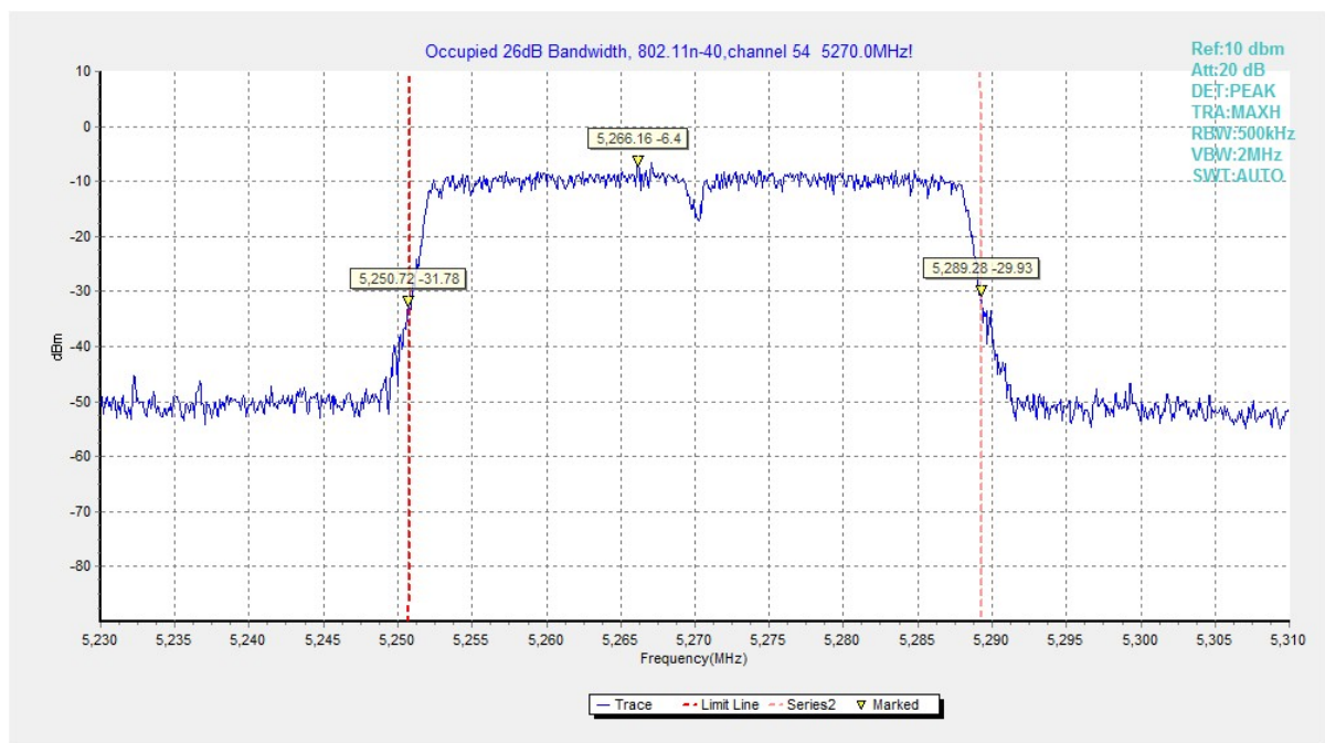
Fig. 30 Occupied 26dB Bandwidth (802.11n40, 5270MHz)
