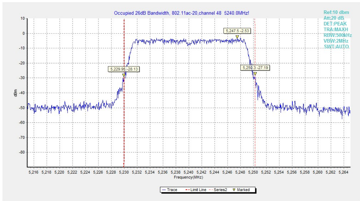
Fig. 21 Occupied 26dB Bandwidth (802.11ac20, 5240MHz)
