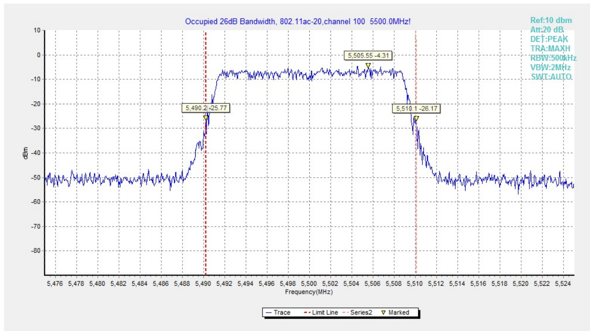
Fig. 25 Occupied 26dB Bandwidth (802.11ac20, 5500MHz)
