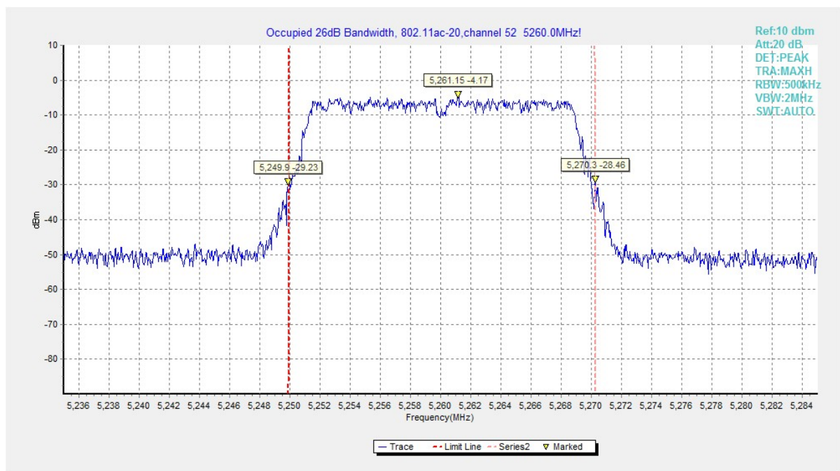
Fig. 22 Occupied 26dB Bandwidth (802.11ac20, 5260MHz)
