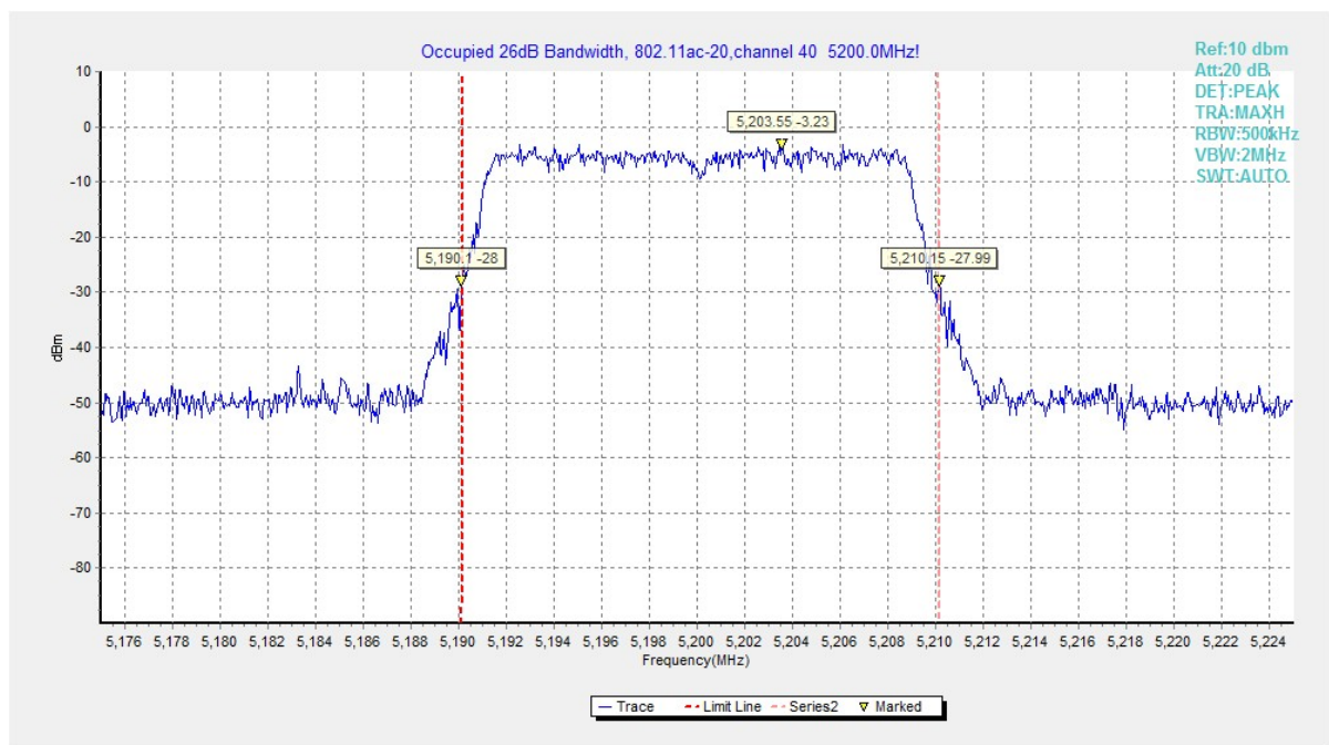
Fig. 20 Occupied 26dB Bandwidth (802.11ac20, 5200MHz)
