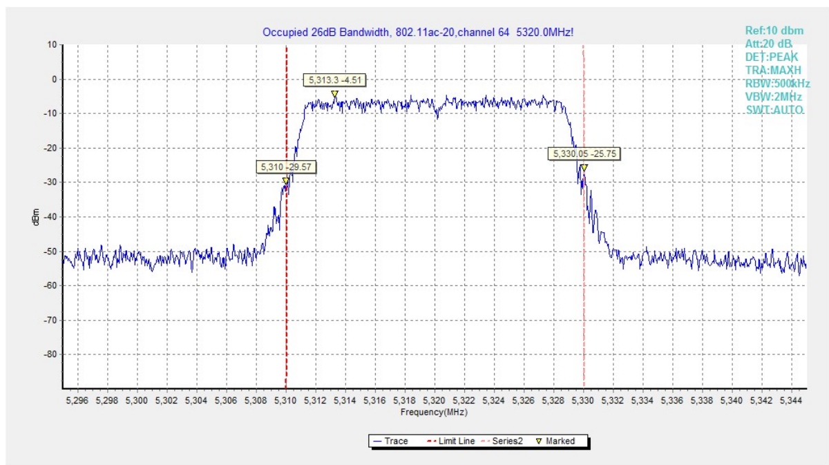
Fig. 24 Occupied 26dB Bandwidth (802.11ac20, 5320MHz)
