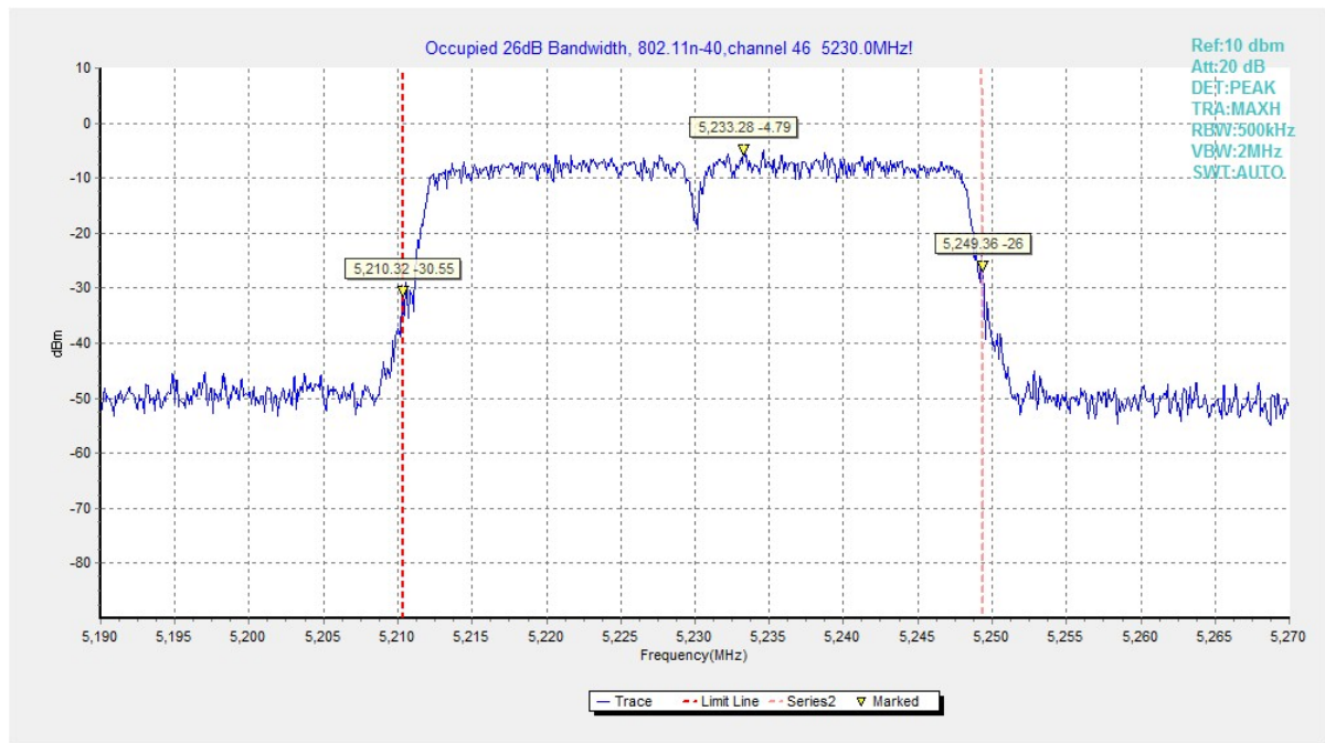
Fig. 29 Occupied 26dB Bandwidth (802.11n40, 5230MHz)
