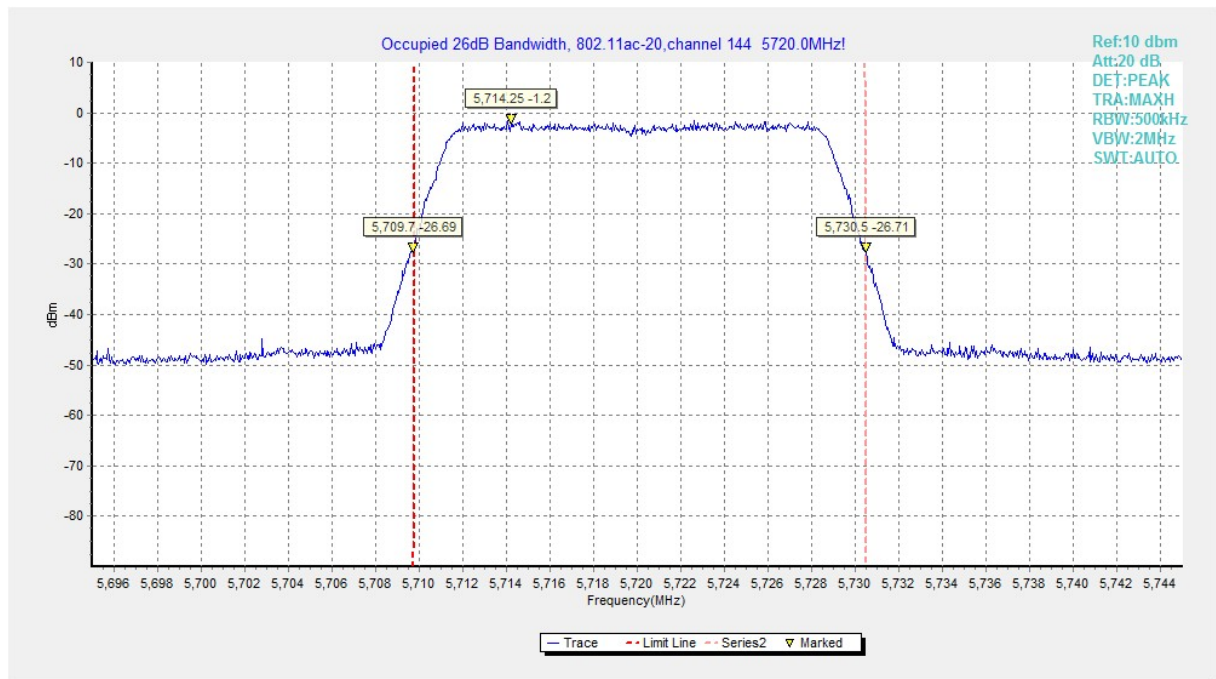
Fig. 27 Occupied 26dB Bandwidth (802.11ac20, 5720MHz)
