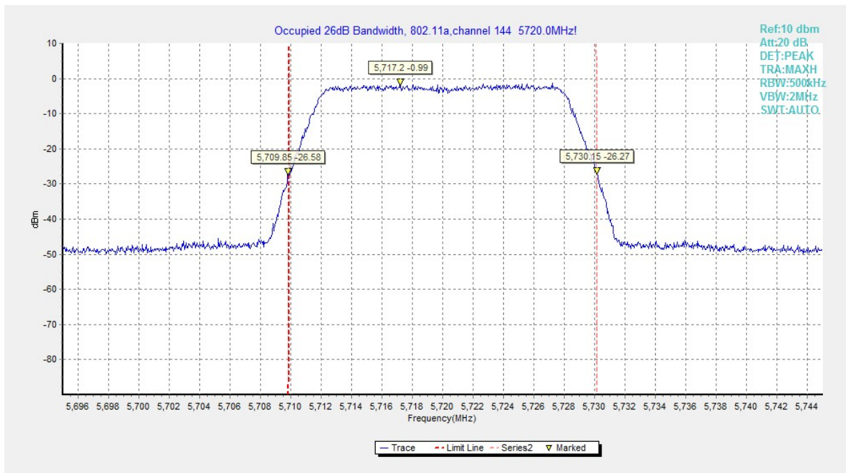
Fig. 9 Occupied 26dB Bandwidth (802.11a, 5720MHz)
