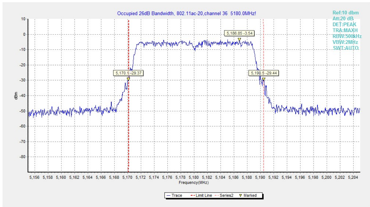
Fig. 19 Occupied 26dB Bandwidth (802.11ac20, 5180MHz)
