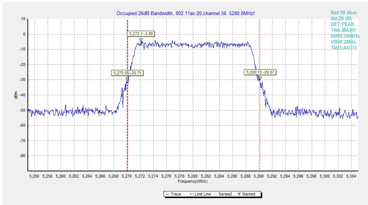
Fig. 23 Occupied 26dB Bandwidth (802.11ac20, 5280MHz)
