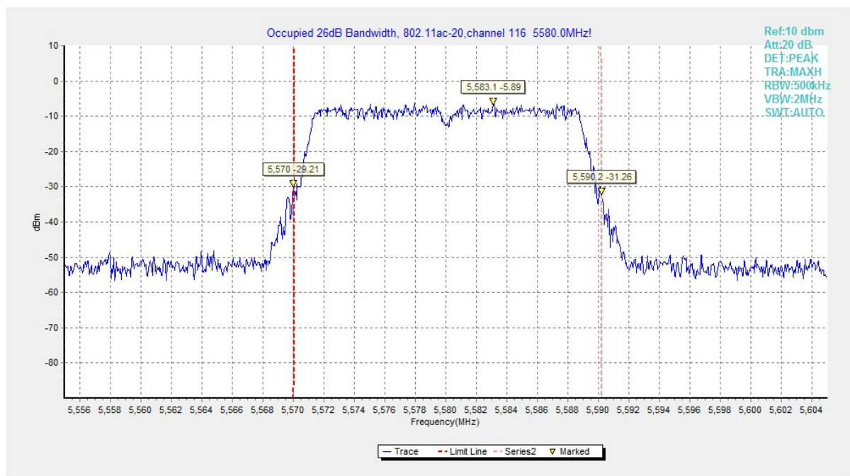
Fig. 26 Occupied 26dB Bandwidth (802.11ac20, 5580MHz)
