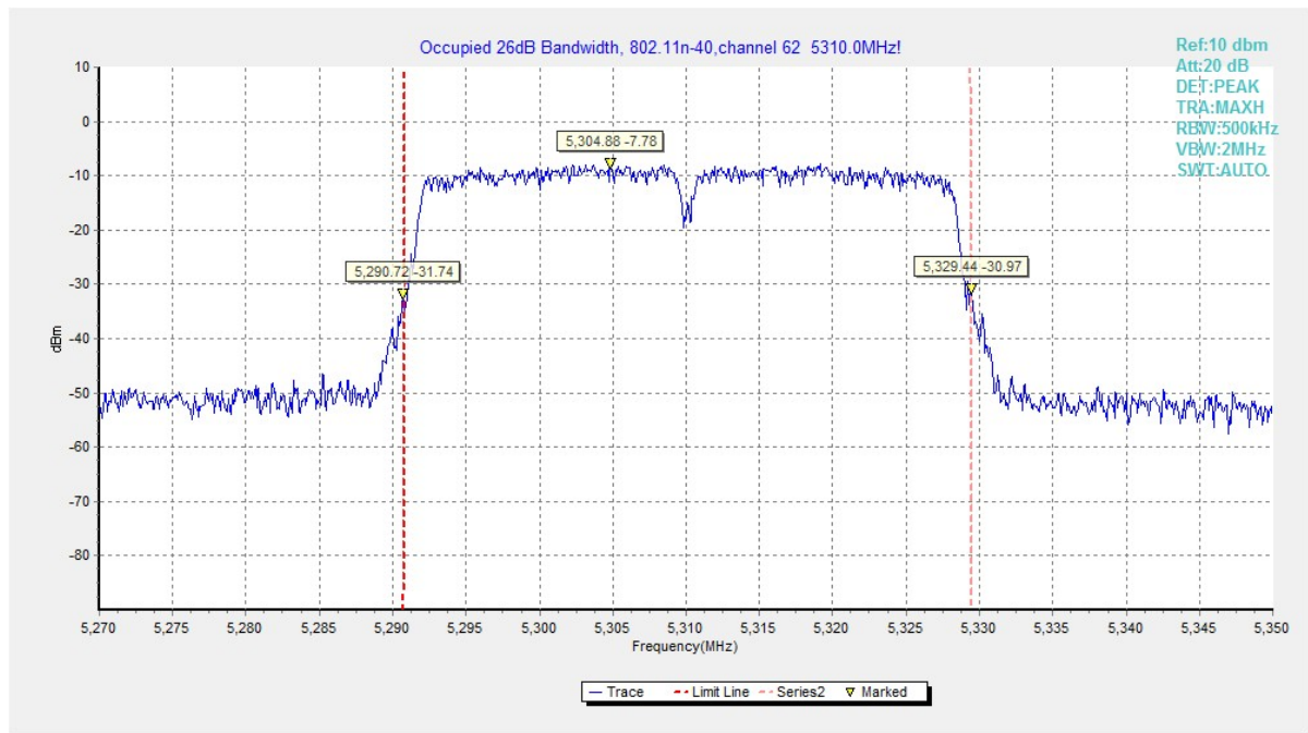
Fig. 31 Occupied 26dB Bandwidth (802.11n40, 5310MHz)
