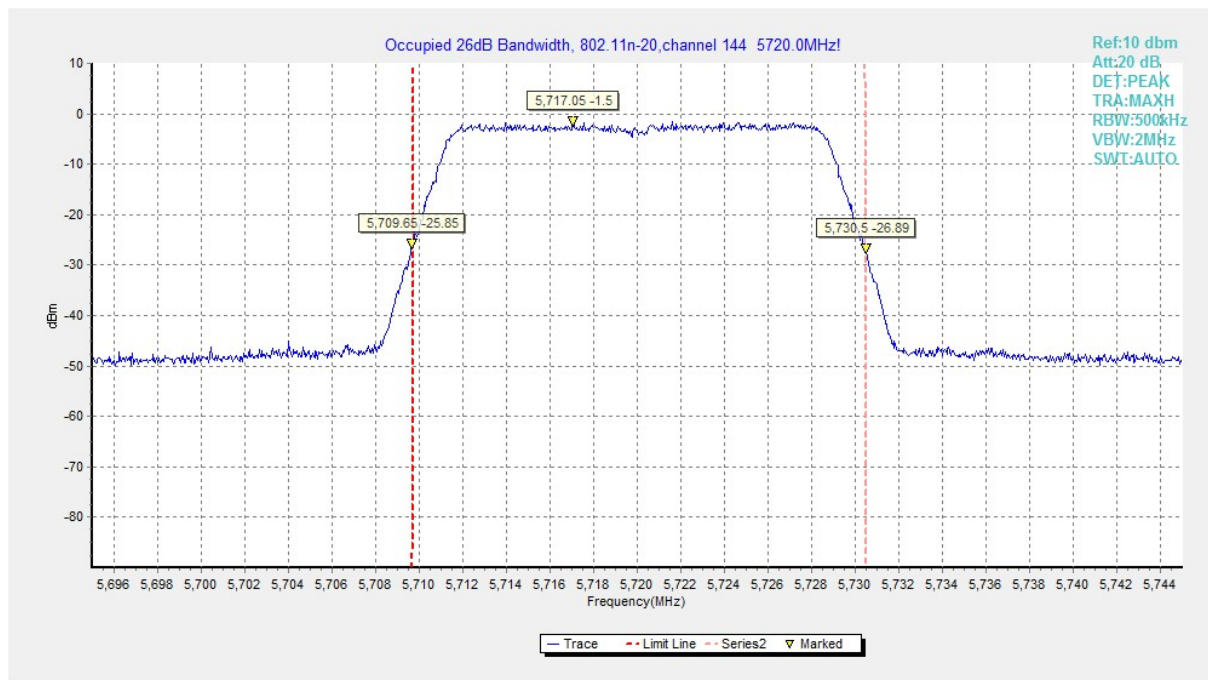
Fig. 18 Occupied 26dB Bandwidth (802.11n20, 5720MHz)
